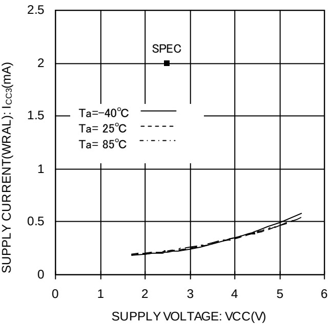
Figure 18. WRAL 動作時消費電流 I_{CC3}(\text{WRAL}, f_{SK}=1\text{MHz})
