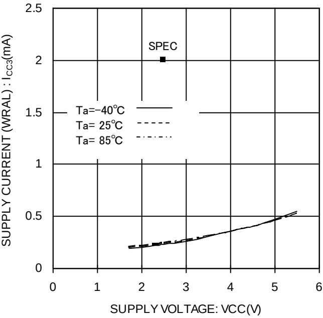
Figure 18. WRAL 動作時消費電流 I_{cc3}(WRAL, f_{sk}=1MHz)
