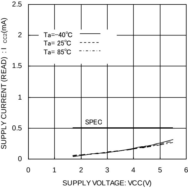
Figure 16. READ 動作時消費電流 I_{cc2}(READ, f_{sk}=1MHz)
