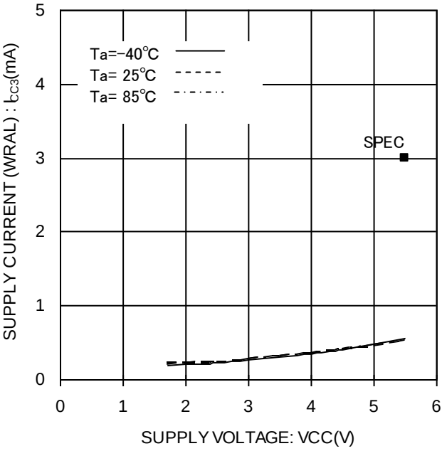
Figure 19. WRAL 動作時消費電流 I_{cc3}(WRAL, f_{sk}=3MHz)
