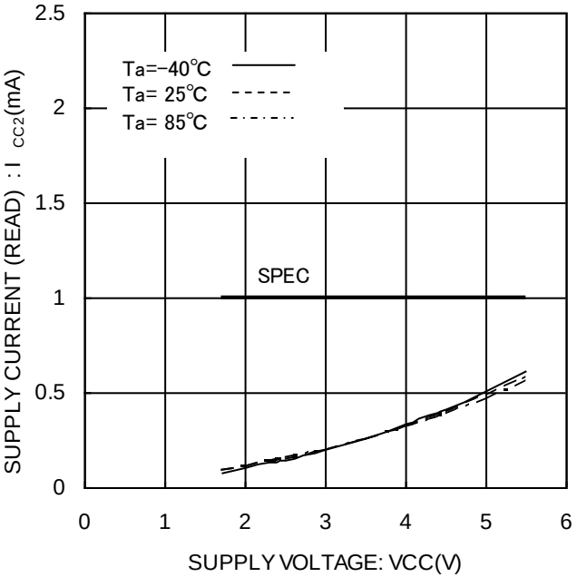
Figure 17. READ 動作時消費電流 I_{cc2}(READ, f_{sk}=3MHz)
