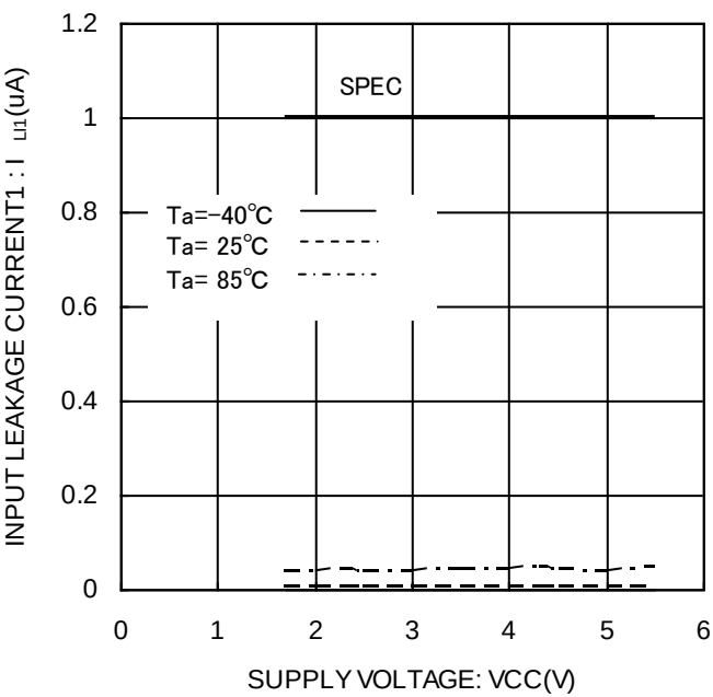
Figure 12. 入力リーク電流 1 I_{LI1}(DI)
