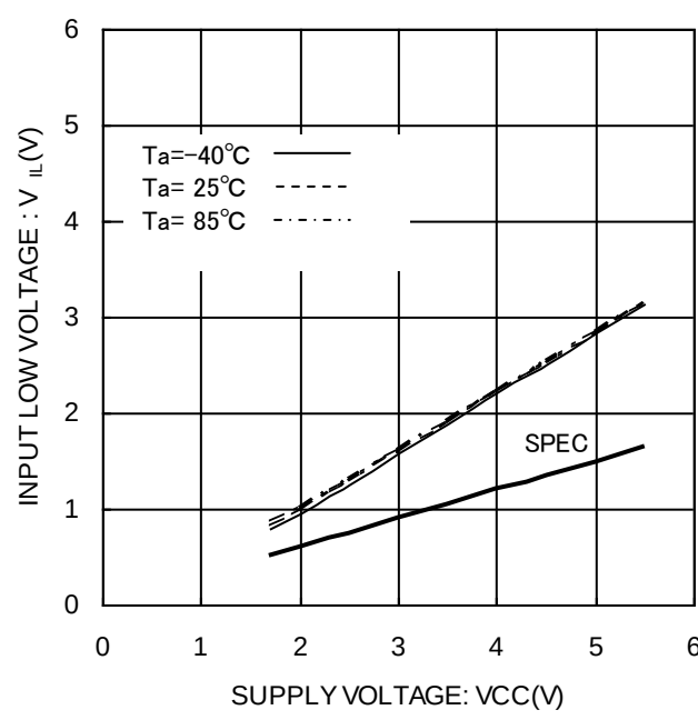
Figure 5.”L”入力電圧 V_{IL} (CS,SK,DI)
