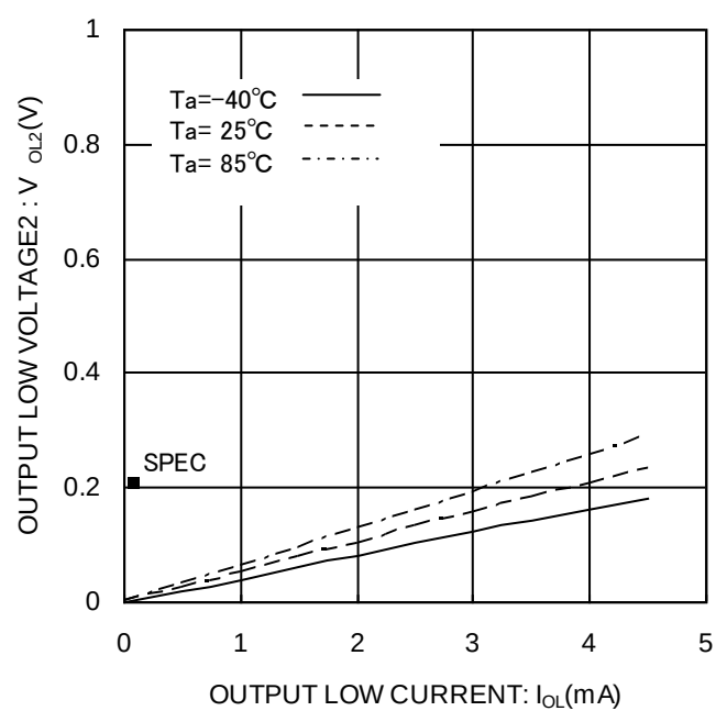
Figure 7. “L”出力電圧 2 V_{OL2} ( V_{CC}=1.7\text{V} )
