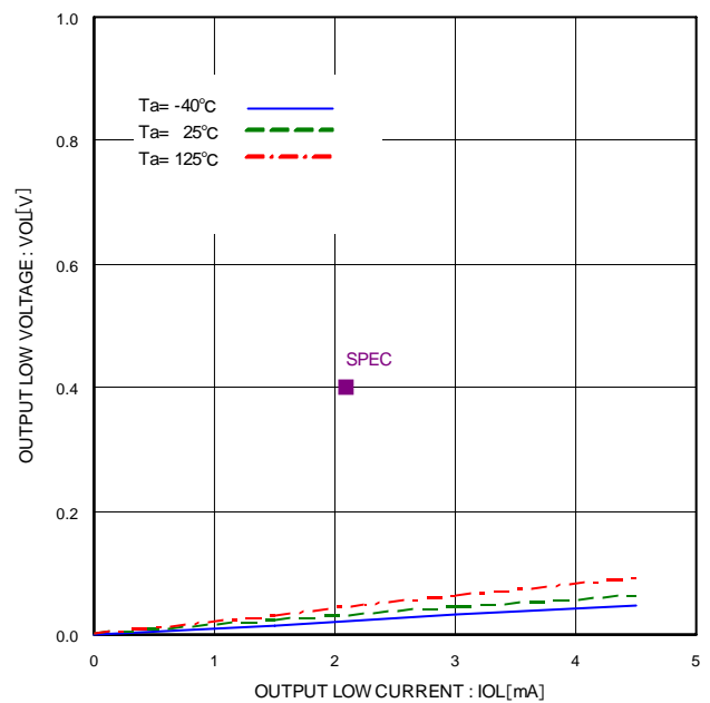
Figure 7. L 出力電圧 V_{OL} - I_{OL} ( V_{CC}=4.0V )
