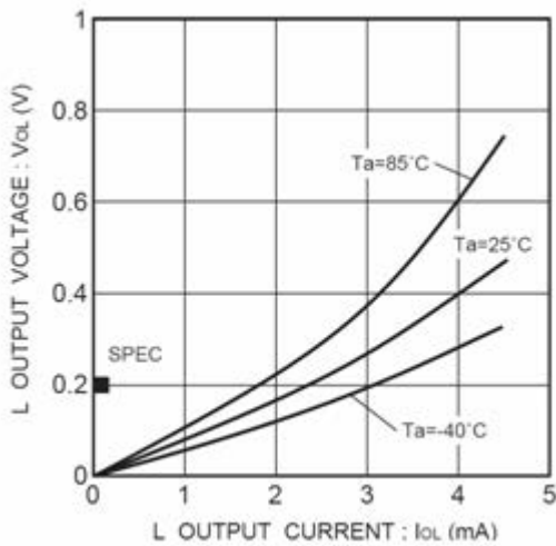
Figure 4. “L”出力電圧 V_{OL} - I_{OL} ( V_{CC}=1.8V )
