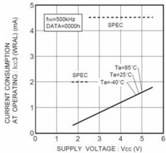
Figure 17. 動作時消費電流 WRAL ICC3 (WRAL, fSK=500kHz)
