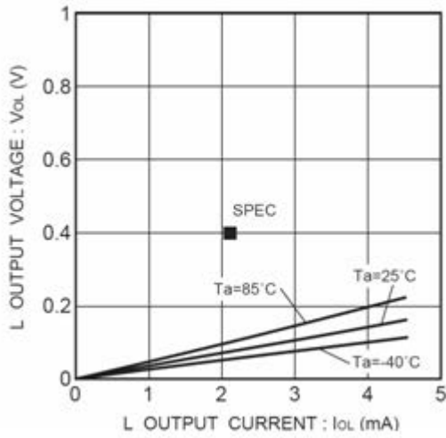
Figure 6. “L”出力電圧 V_{OL} - I_{OL} ( V_{CC}=4.0\text{V} )
