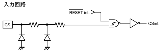
Figure 45. 入力回路(CS)
