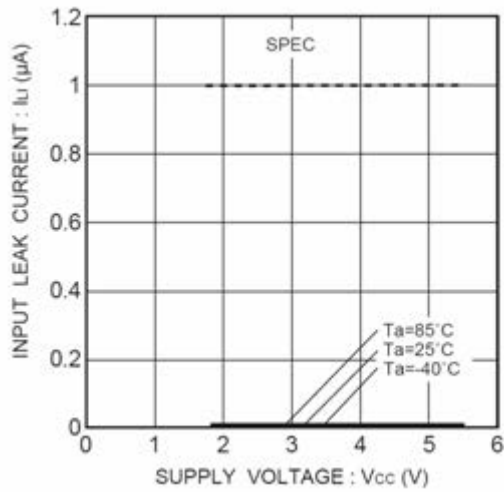
Figure 10. 入力リーク電流 ILI (CS,SK,DI)
