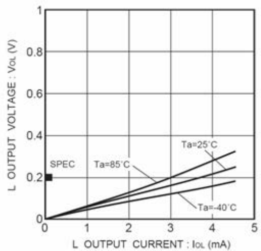
Figure 5. “L”出力電圧 V_{OL} - I_{OL} ( V_{CC}=2.5V )
