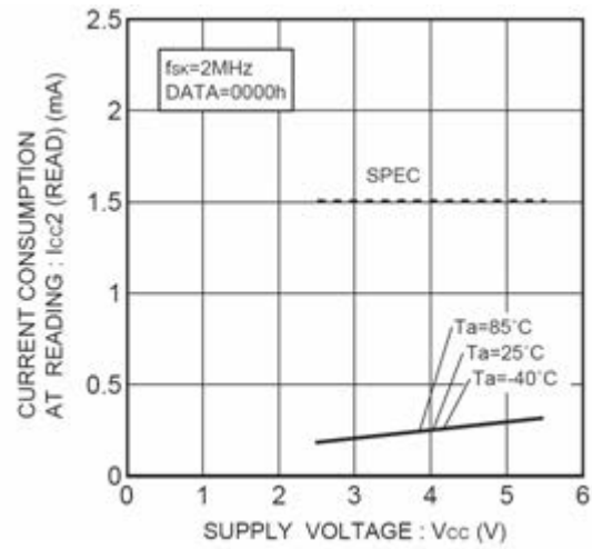
Figure 13. 動作時消費電流 READ ICC2 (READ, fSK=2MHz)
