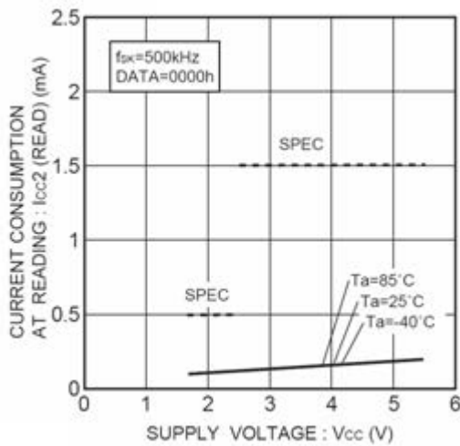
Figure 16. 動作時消費電流 READ ICC2 (READ, fSK=500kHz)
