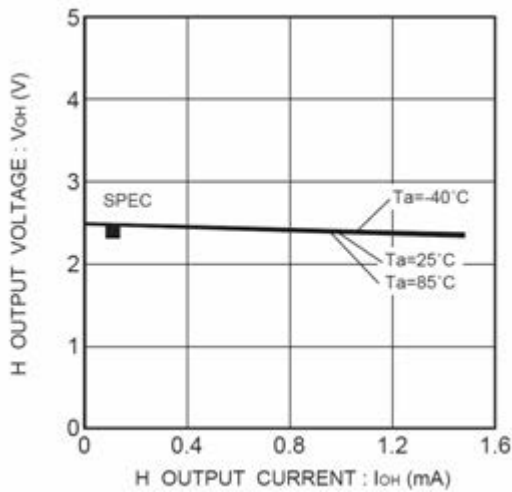
Figure 8. “H”出力電圧 V_{OH} - I_{OH} ( V_{CC}=2.5\text{V} )
