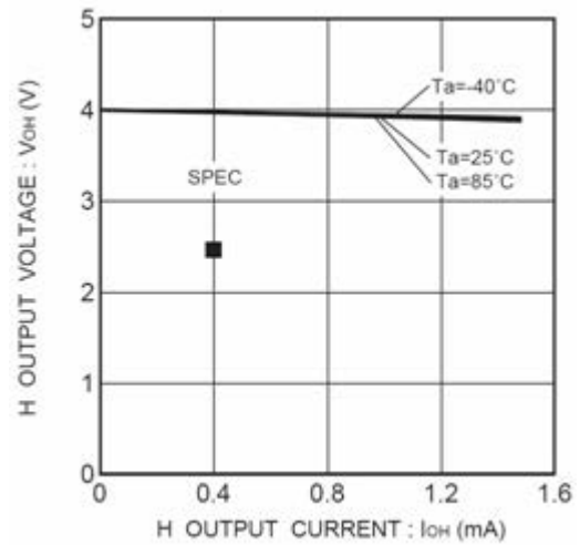
Figure 9. “H”出力電圧 V_{OH} - I_{OH} ( V_{CC}=4.0\text{V} )
