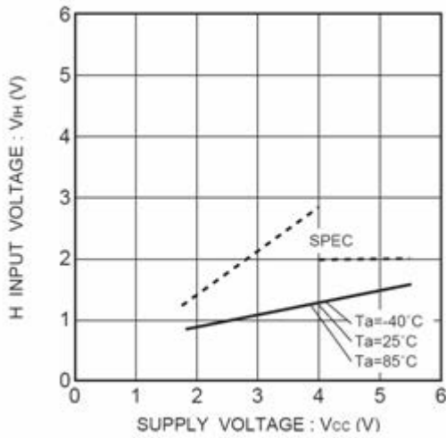
Figure 2. “H”入力電圧 V_{IH} (CS,SK,DI)
