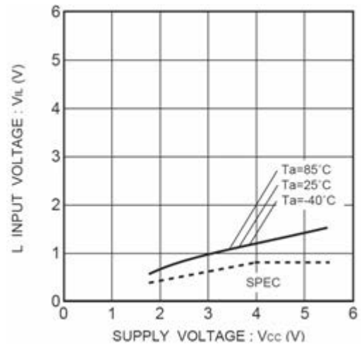
Figure 3. “L”入力電圧 V_{IL} (CS,SK,DI)
