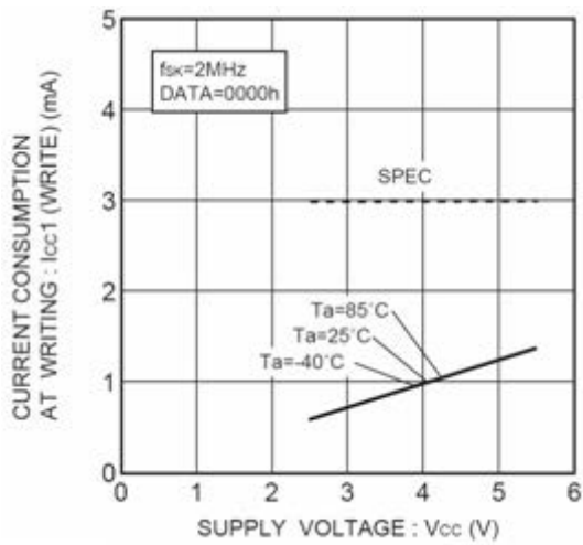
Figure 12. 動作時消費電流 WRITE ICC1 (WRITE, fSK=2MHz)
