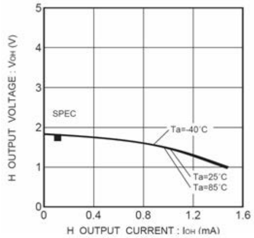
Figure 7. “H”出力電圧 V_{OH} - I_{OH} ( V_{CC}=1.8\text{V} )
