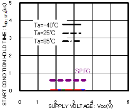
Figure 14. Start Condition Hold Time t_{HD:STA}
