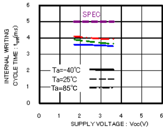
Figure 21. Internal writing cycle time t_{WR}
