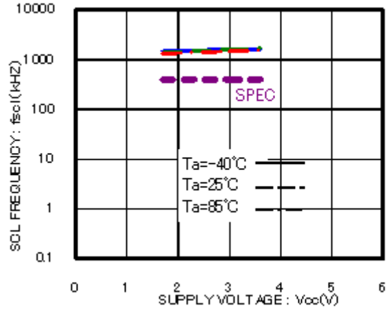
Figure 11. SCL frequency f_{scl}
