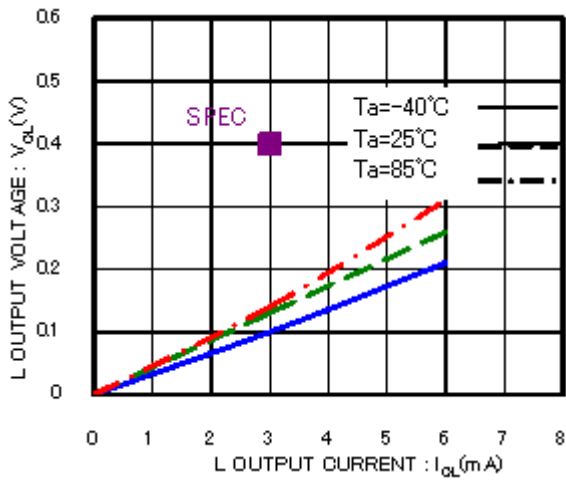
Figure 4. 'L' output voltage V_{OL-I_{OL}} ( V_{CC}=2.5V )
