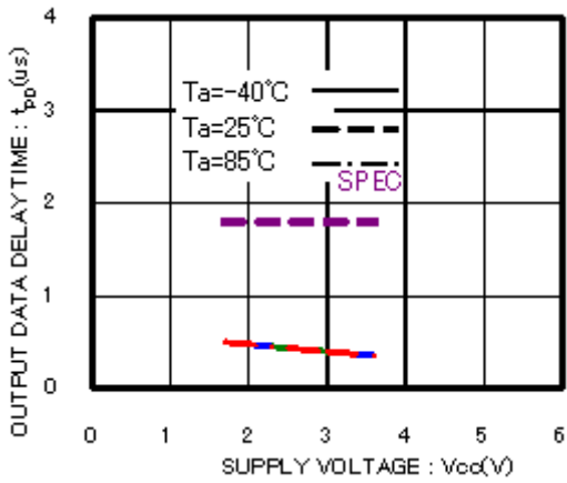
Figure 18. 'L' Data output delay time t_{PD0}
