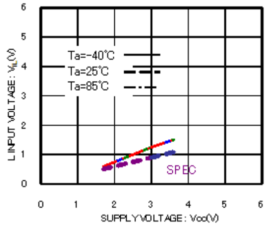
Figure 3. 'L' input voltage V_{IL} (SCL,SDA,WP)
