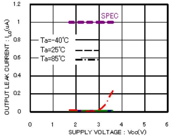
Figure 7. Output leak current I_{LO} (SDA)
