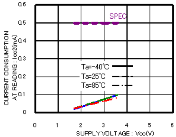
Figure 9. Current consumption at READ operation I_{cc2} (fscI=400kHz)
