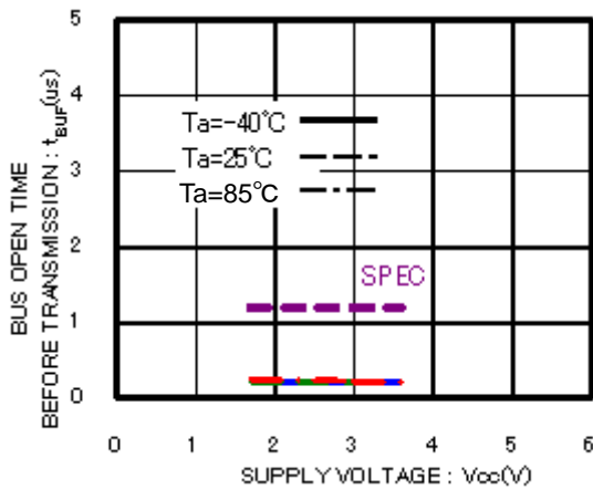
Figure 20. BUS open time before transmission t_{BUF}
