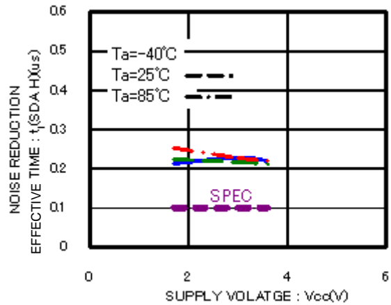
Figure 23. Noise reduction effective time t_1(\text{SDA H})
