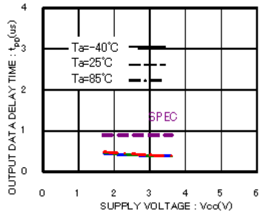
Figure 19. 'H' Data output delay time t_{PD1}
