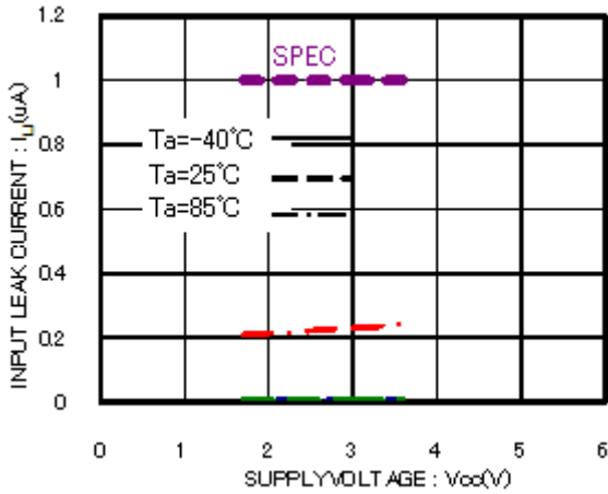
Figure 6. Input leak current I_{LI} (SCL,WP)
