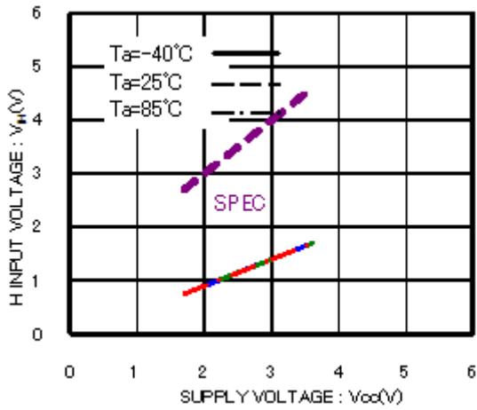
Figure 2. 'H' input voltage V_{IH} (SCL,SDA,WP)
