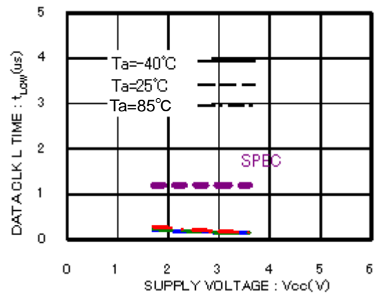
Figure 13. Data clock Low Period t_{LOW}
