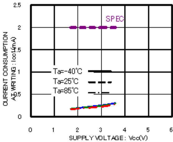
Figure 8. Current consumption at WRITE operation I_{cc1} (fscI=400kHz)
