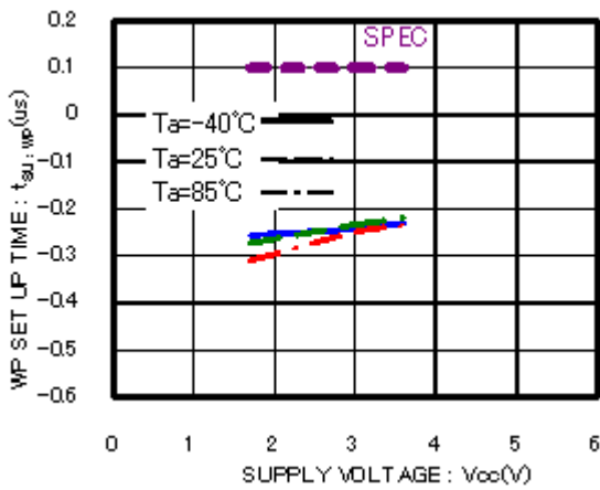
Figure 24. WP setup time t_{\text{SU:WP}}
