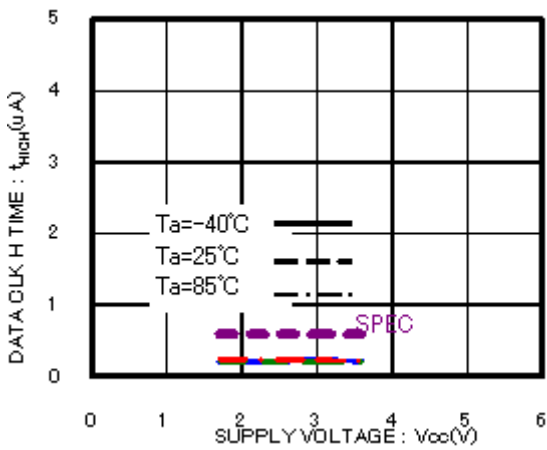
Figure 12. Data clock High Period t_{HIGH}
