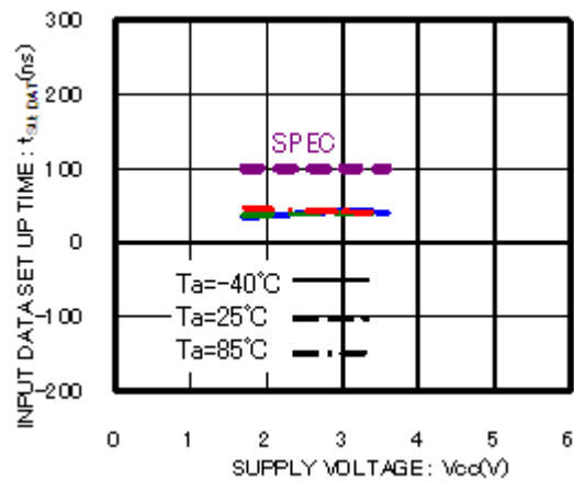
Figure 17. Input Data Setup Time t_{SU:DAT} (HIGH)
