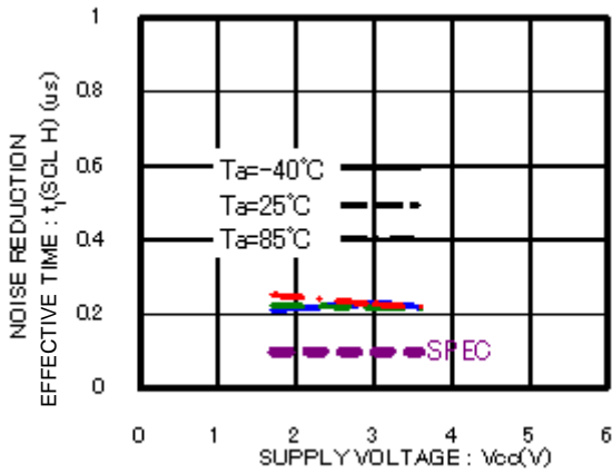
Figure 22. Noise reduction effective time t_1(\text{SCL H})
