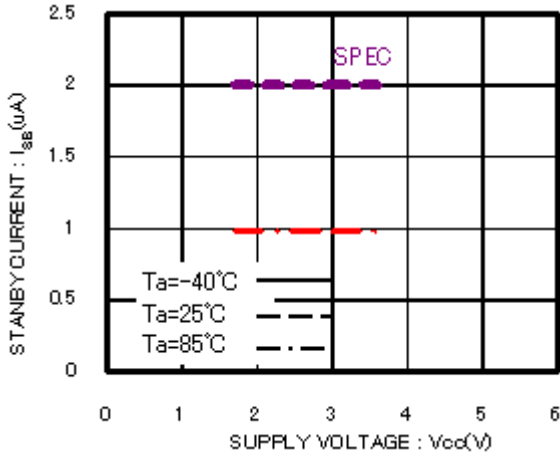
Figure 10. Standby operation I_{SB}
