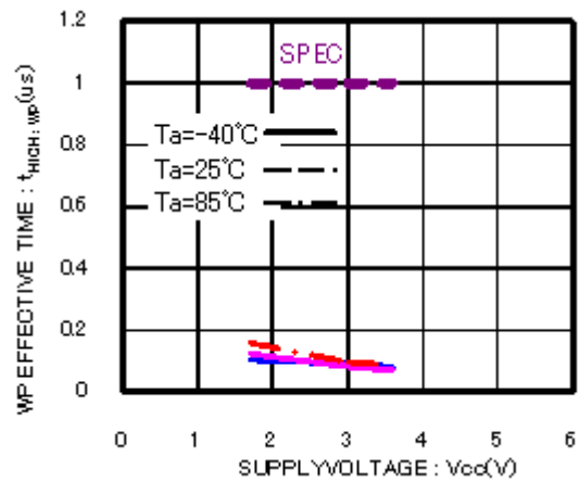
Figure 25. WP effective time t_{\text{HIGH:WP}}
