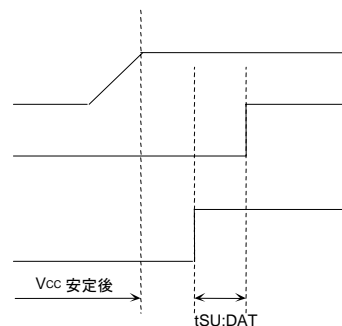
Figure 46. SCL='H' SDA='L'の時
