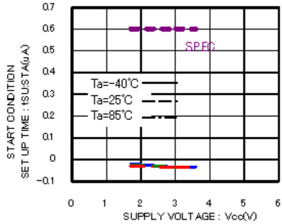
Figure 15. Start Condition Setup Time t_{SU:STA}
