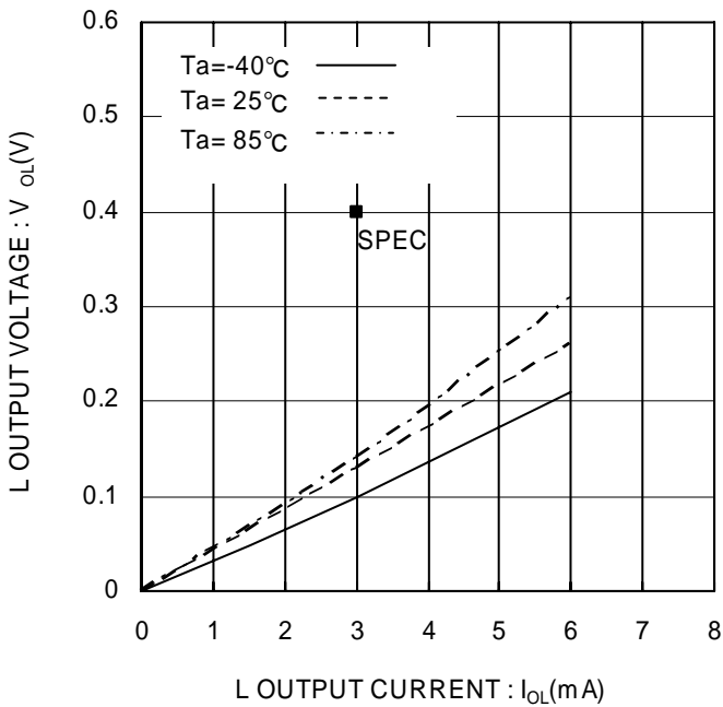
Figure 5. “L”出力電圧 V_{OL-I_{OL}} ( V_{CC}=1.7V )
