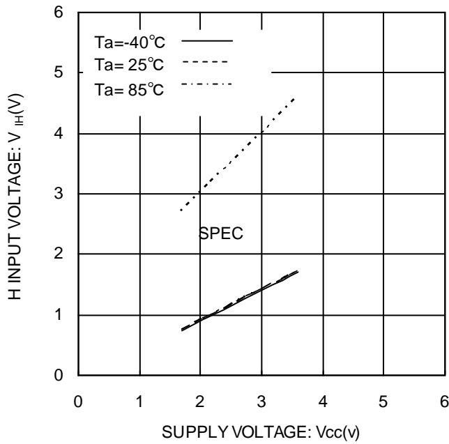
Figure 3. “H”入力電圧 V_{IH} (SCL,SDA)
