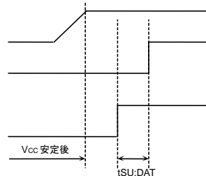
Figure 48. SCL='H' SDA='L'の時
