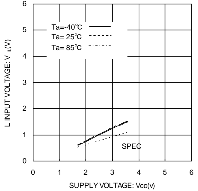
Figure 4. “L”入力電圧 V_{IL} (SCL,SDA)
