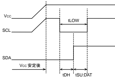
Figure 47. SCL='H' SDA='L'の時
