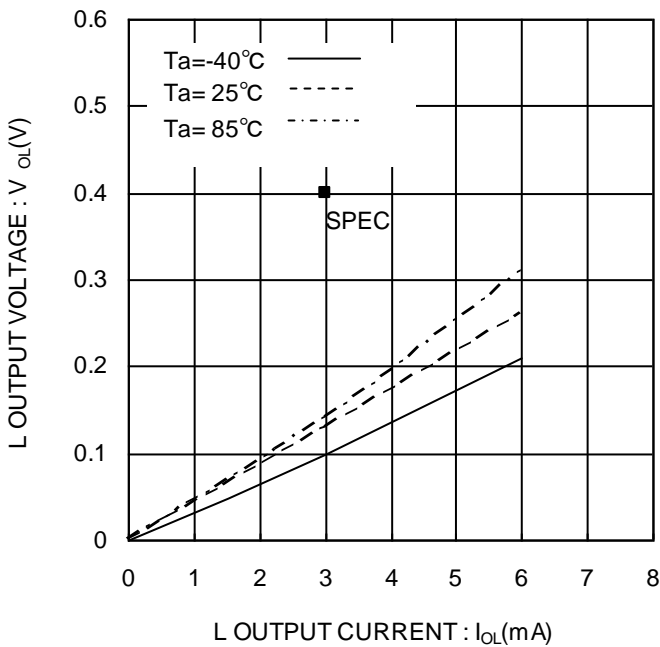
Figure 5. “L”出力電圧 V_{OL-I_{OL}} ( V_{CC}=1.7V )
