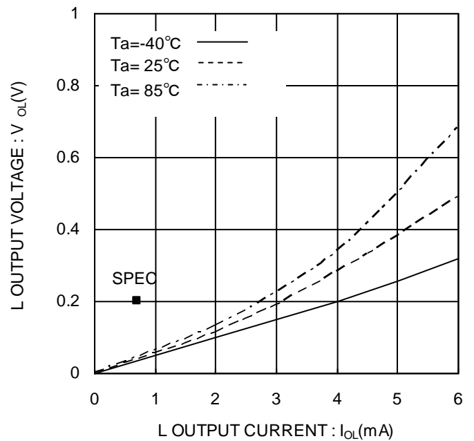
Figure 6. “L”出力電圧 V_{OL-I_{OL}} ( V_{CC}=2.5V )
