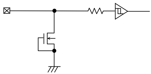
Figure 50. 入力端子回路図 (SCL)
