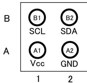
Figure 3. 端子配置図(bottom view)
