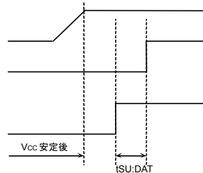
Figure 50. SCL='H' SDA='L'の時
