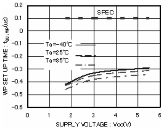
Figure 28. WP setup time t_{SU:WP}
