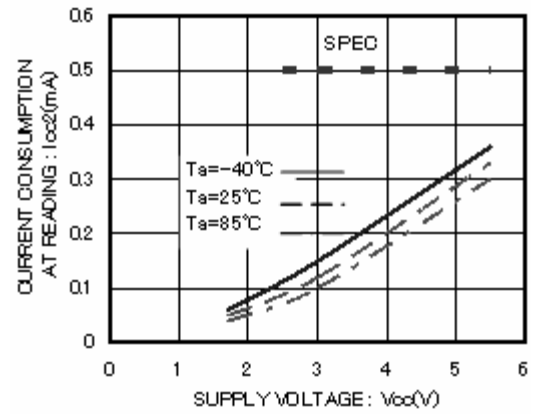
Figure 9. Current consumption at READ operation I_{CC2} (fsc2=400kHz)
