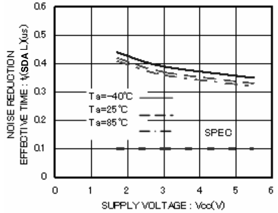
Figure 27. Noise reduction effective time t_1 (SDA L)
