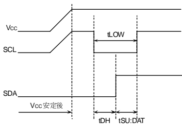
Figure 49. SCL='H' SDA='L'の時
