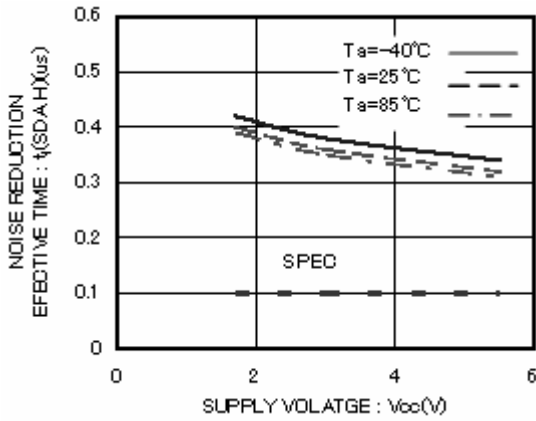
Figure 26. Noise reduction effective time t_1 (SDA H)
