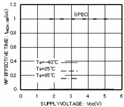
Figure 29. WP effective time t_{HIGH:WP}
