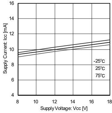
Fig.1 回路電流 (BA6247FP-Y)
