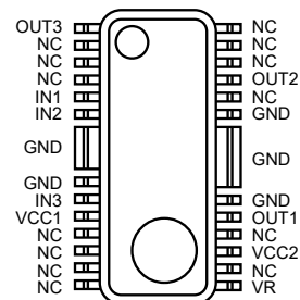
Fig.10 BA6247FP-Y (HSOP25)
