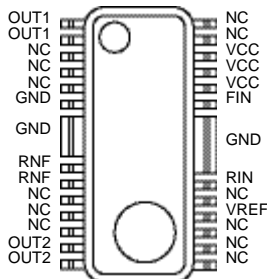
Figure 6. HSOP25(TOP VIEW)
