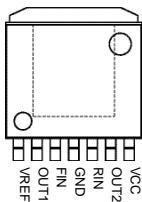
Figure 4. HRP7(TOP VIEW)
