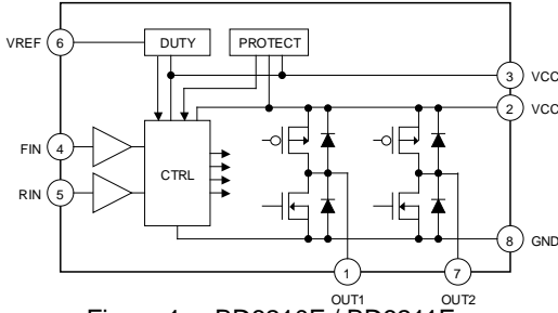
Figure 1. BD6210F / BD6211F
