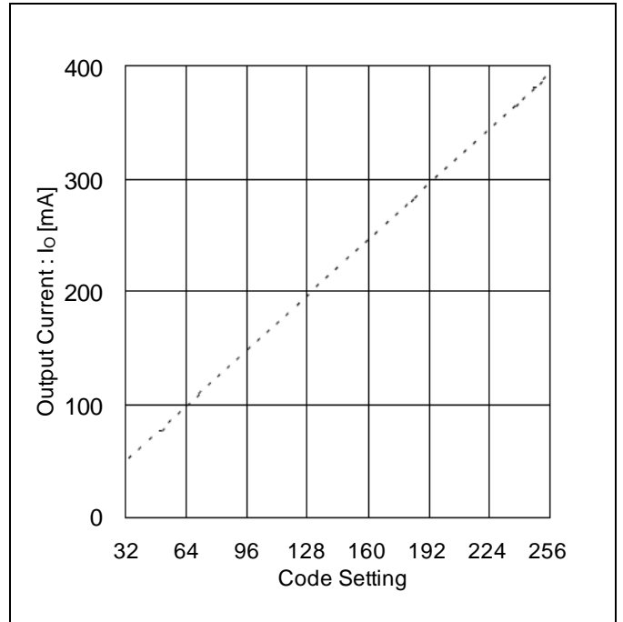
Figure 12. Output Current vs Code Setting (Current Driver Block, R RNF =1.0 Ω, R L =5.0 Ω)
