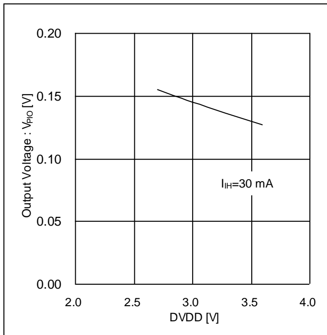
Figure 13. Output Voltage vs DVDD (PIOUT1 Driver Circuit)
