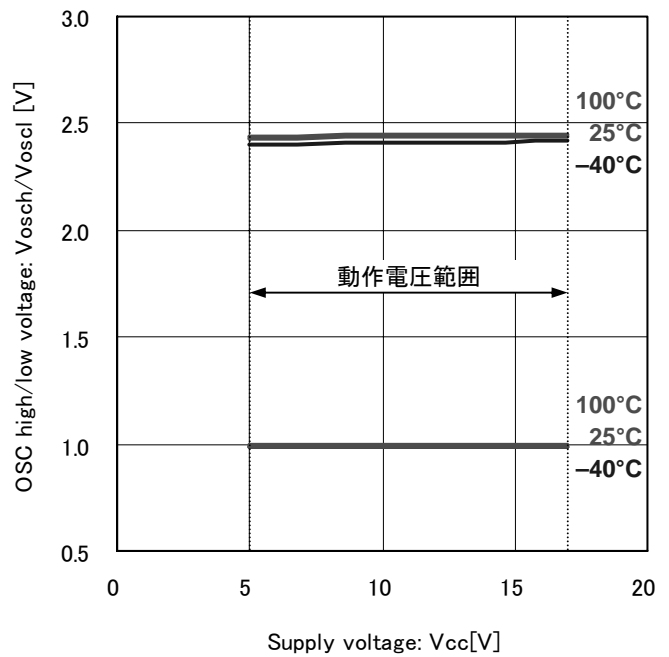
Fig.14 OSC High/Low 電圧
