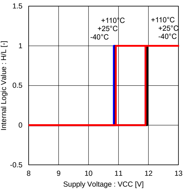
Figure 45. 下側 UVLO 特性
