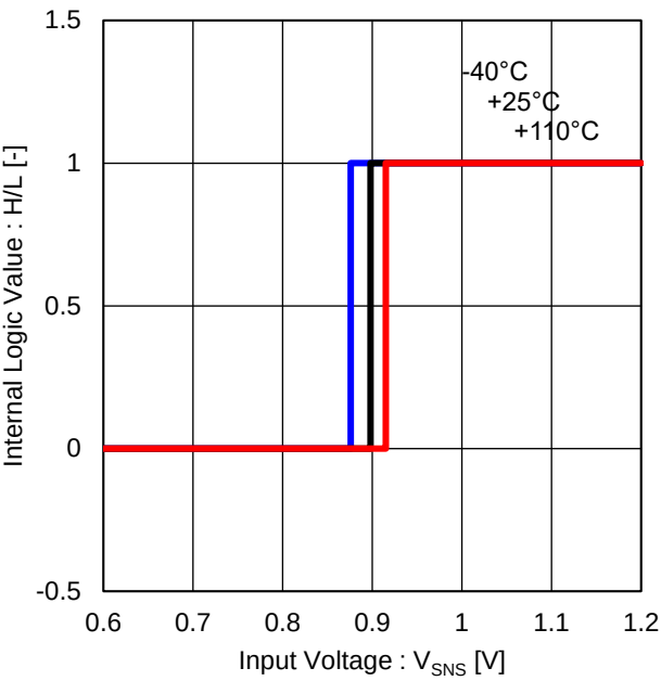
Figure 42. 過電流検出電圧 (SNS)
