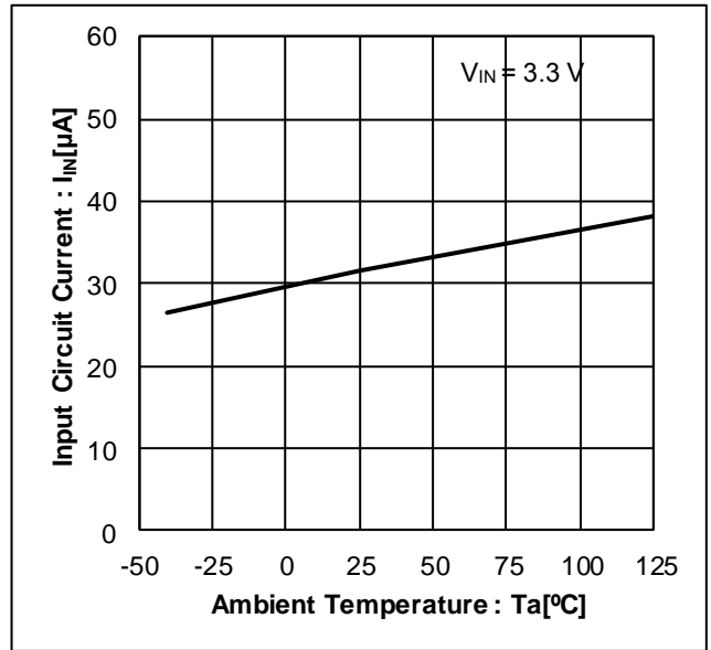
Figure 6. Input Circuit Current vs Ambient Temperature ( V_{IN} = 3.3\text{ V} )
