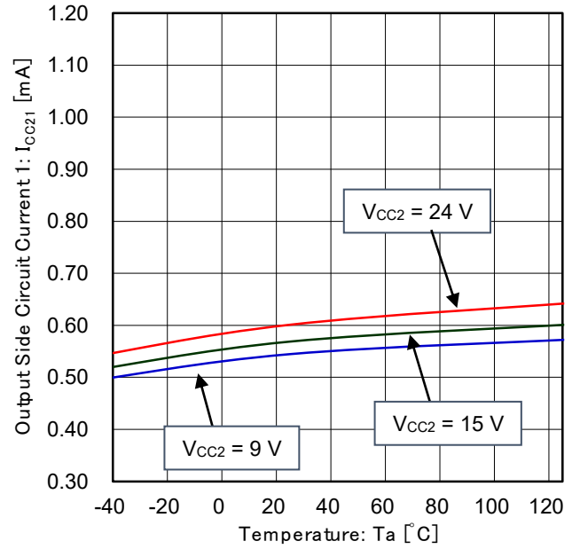
Figure 8. Output Side Circuit Current 1 vs Temperature (OUT = L 時)
