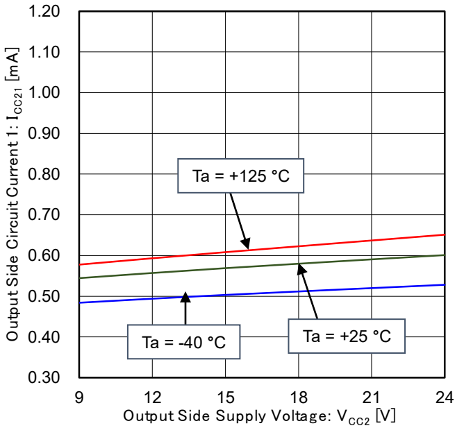
Figure 7. Output Side Circuit Current 1 vs Output Side Supply Voltage (OUT = L 時)
