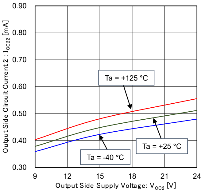
Figure 9. Output Side Circuit Current 2 vs Output Side Supply Voltage (OUT = H 時)
