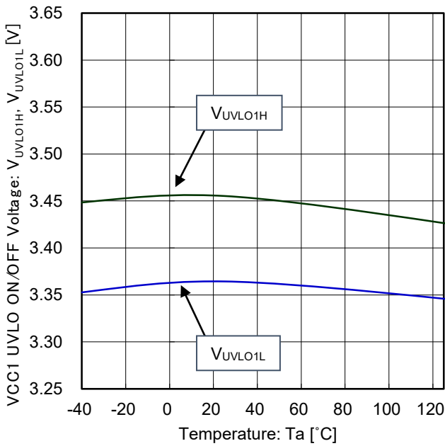
Figure 21. VCC1 UVLO ON/OFF Voltage vs Temperature
