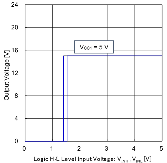
Figure 12. Output Voltage vs Logic H/L Level Input Voltage (V CC1 = 5 V, V CC2 = 15 V, Ta = 25 °C)
