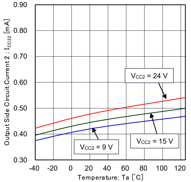
Figure 10. Output Side Circuit Current 2 vs Temperature (OUT = H 時)
