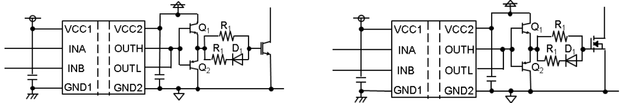
Figure 28. IGBT or MOSFET 駆動時
