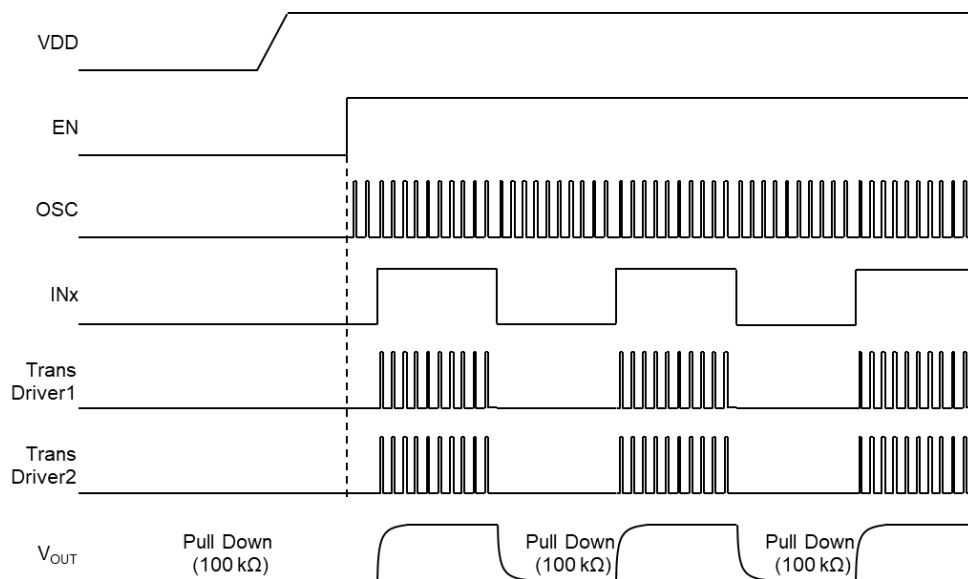
Figure 17. Timing Chart
