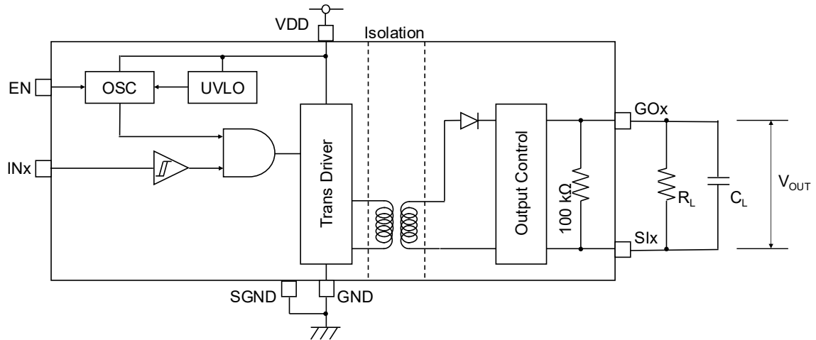
Figure 16. Block Diagram
