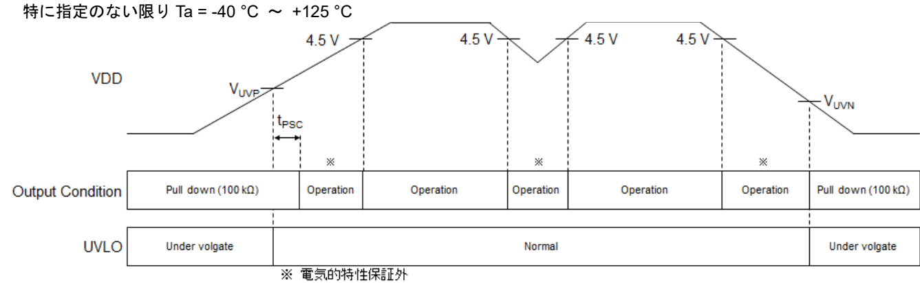
Figure 13. Power Supply Sequence Chart
