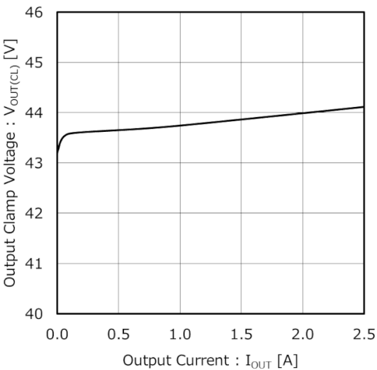
Figure 8. Output Clamp Voltage vs Output Current
