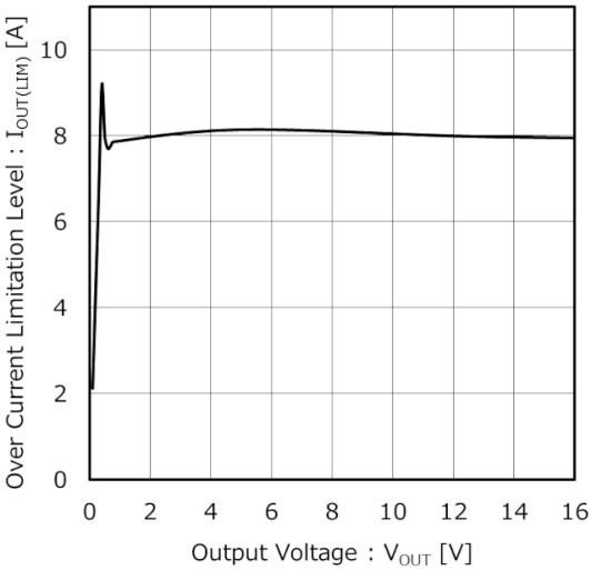
Figure 18. Over Current Limitation Level vs Output Voltage
