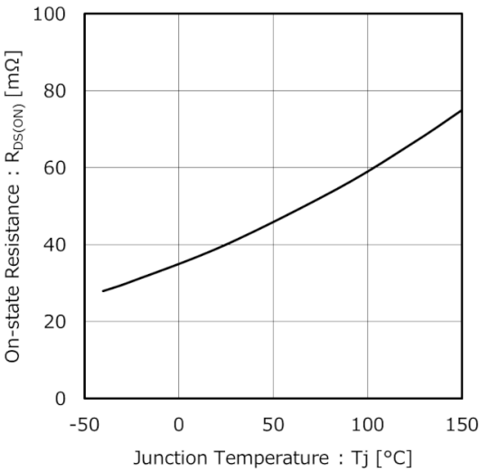
Figure 7. On-state Resistance vs Junction Temperature
