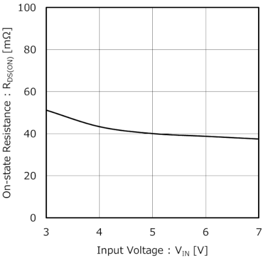
Figure 6. On-state Resistance vs Input Voltage
