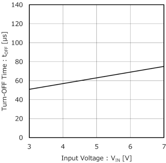
Figure 11. Turn-OFF Time vs Input Voltage
