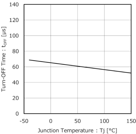
Figure 13. Turn-OFF Time vs Junction Temperature
