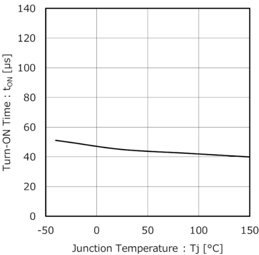
Figure 12. Turn-ON Time vs Junction Temperature
