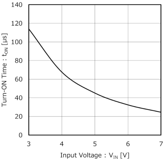
Figure 10. Turn-ON Time vs Input Voltage
