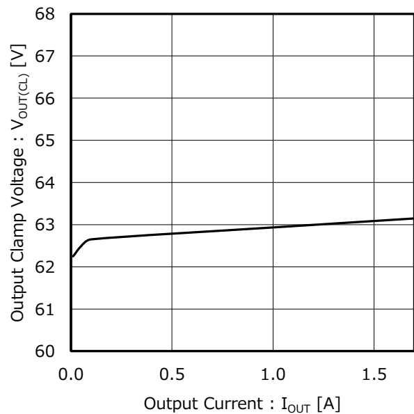
Figure 8. Output Clamp Voltage vs Output Current
