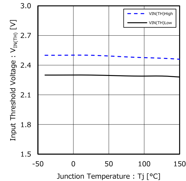
Figure 2. Input Threshold Voltage vs Junction Temperature
