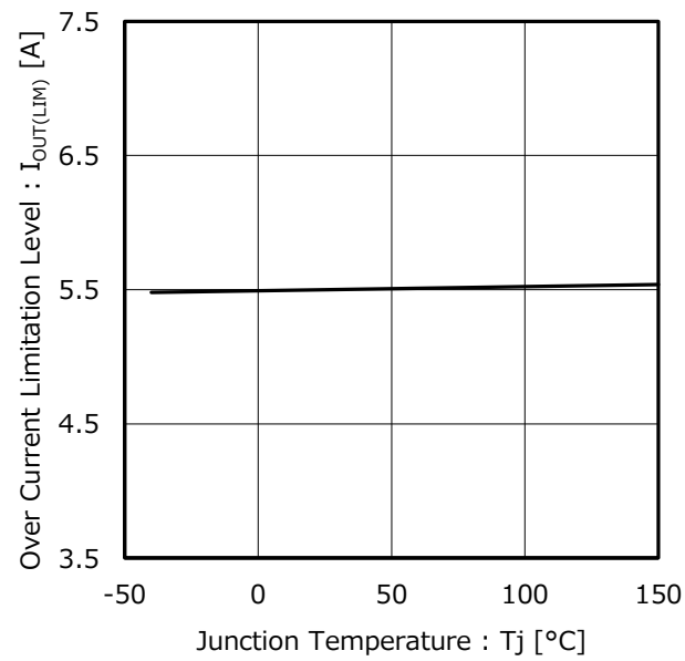
Figure 19. Over Current Limitation Level vs Junction Temperature ( V_{OUT} = 12\text{ V}, 24\text{ V} )
