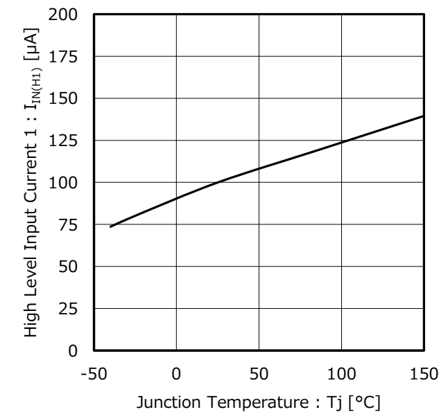
Figure 4. High Level Input Current 1 vs Junction Temperature
