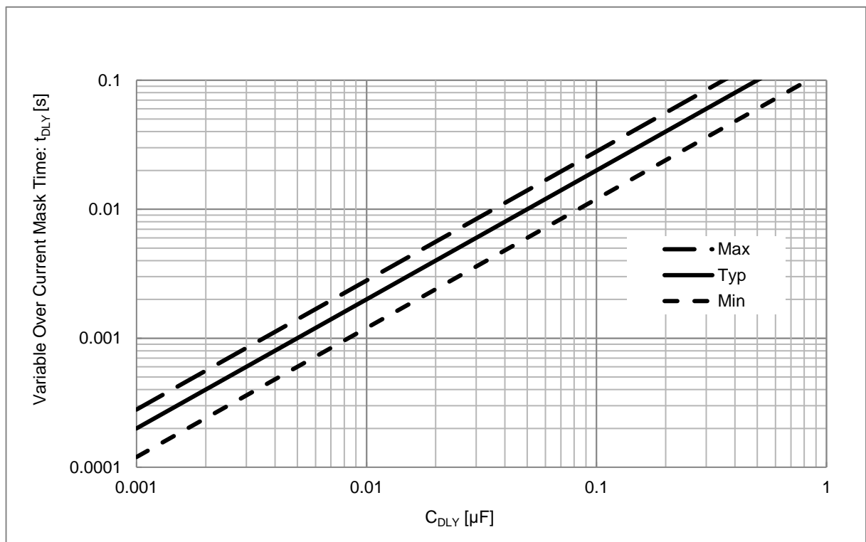
Figure 36. Variable Over Current Mask Time vs C DLY
