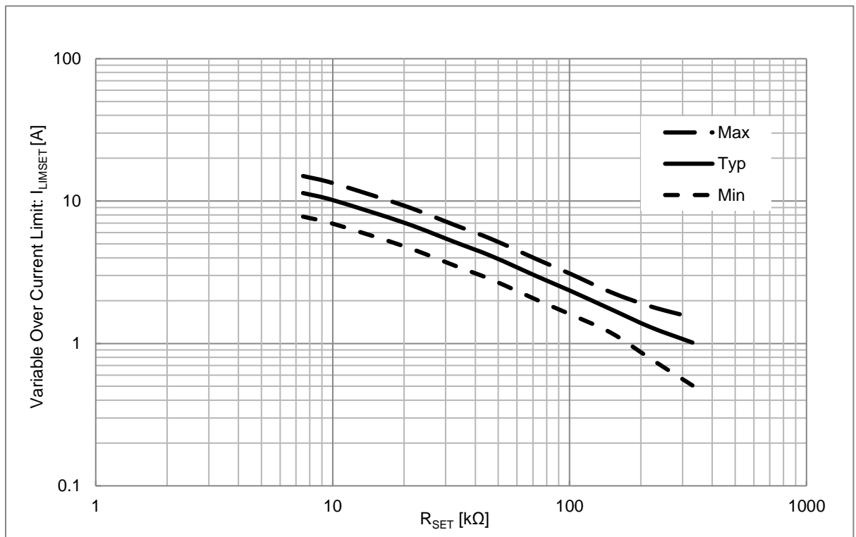
Figure 35. Variable Over Current Limit vs R_{SET}
