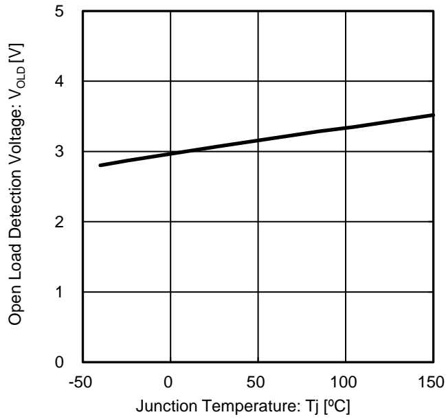
Figure 23. Open Load Detection Voltage vs Junction Temperature
