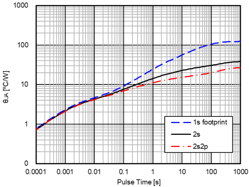
Figure 5. 過渡熱抵抗
