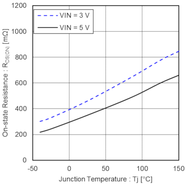
Figure 4. On-state Resistance vs Junction Temperature
