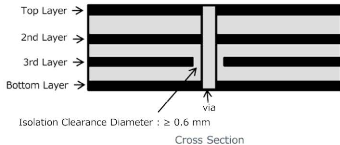
Cross Section
