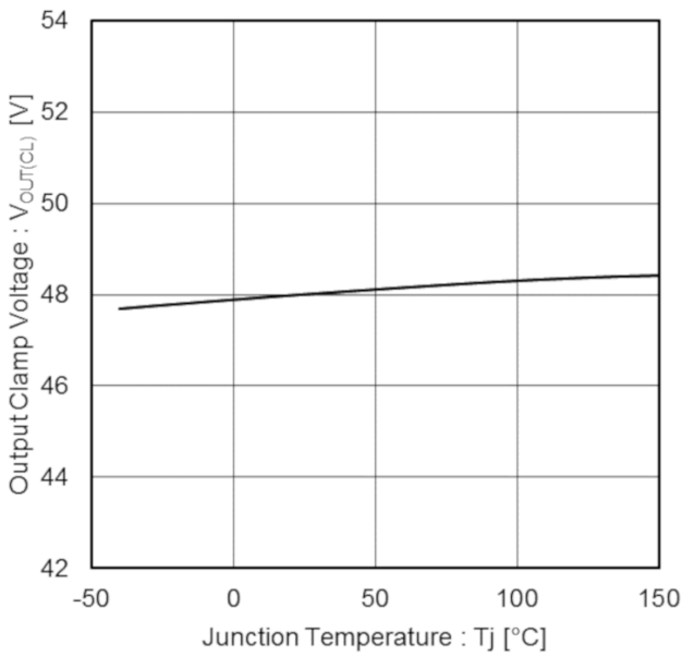
Figure 2. Output Clamp Voltage vs Junction Temperature
