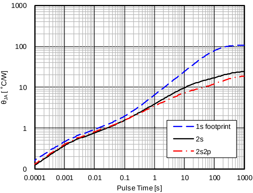
Figure 7. 過渡熱抵抗
