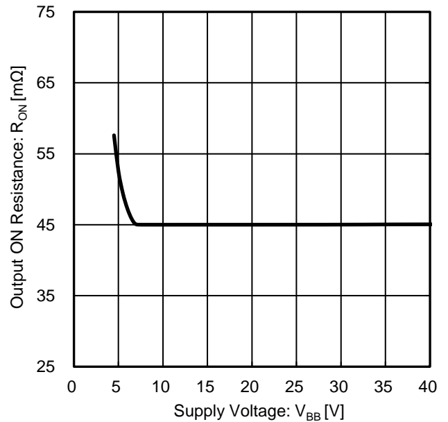
Figure 13. Output ON Resistance vs Supply Voltage
