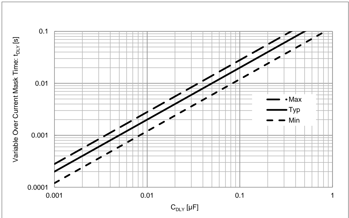
Figure 37. Variable Over Current Mask Time vs C DLY
