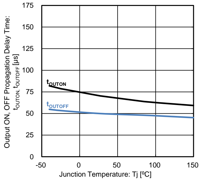
Figure 17. Output ON, OFF Propagation Delay Time vs Junction Temperature
