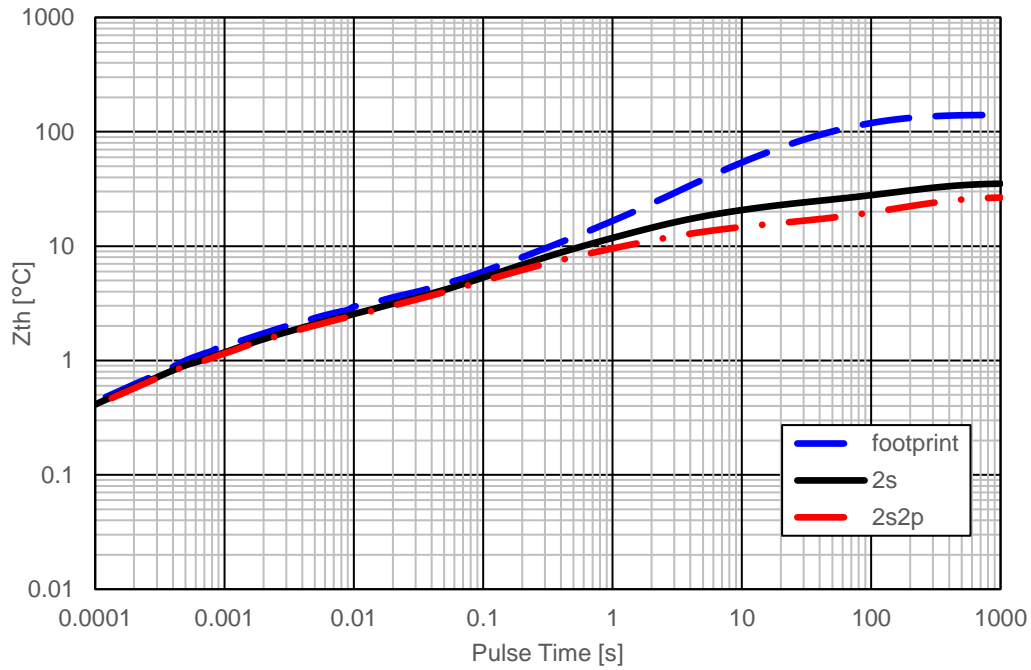
Figure 5. 過渡熱抵抗
