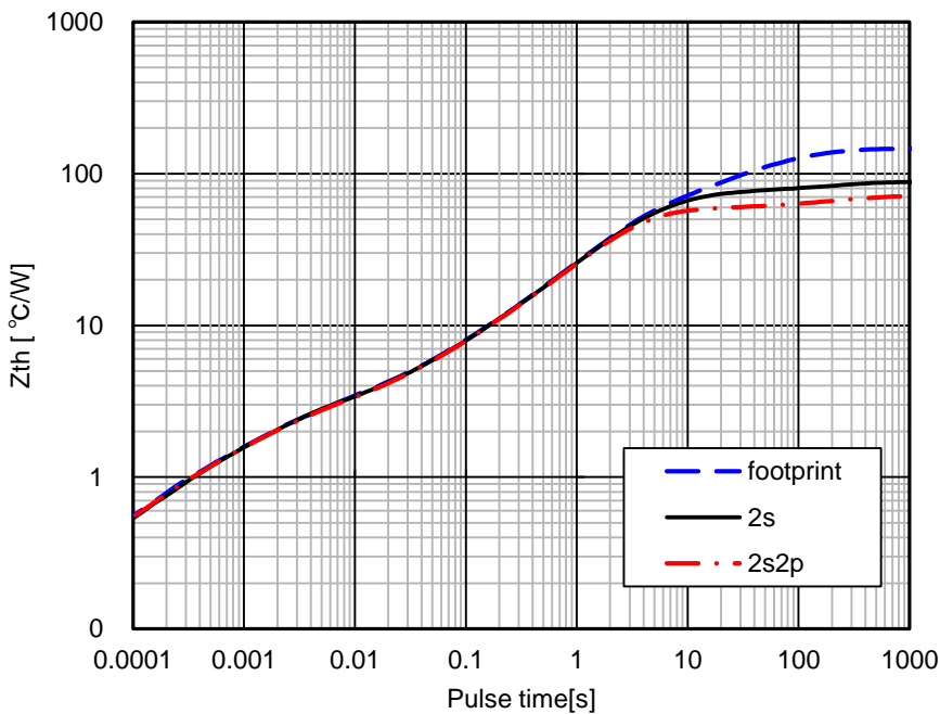
Figure 9. 過渡熱抵抗
