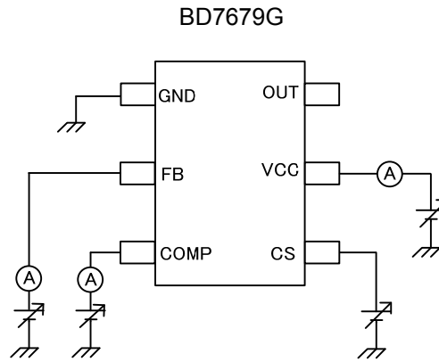
Figure 27, 測定回路図
