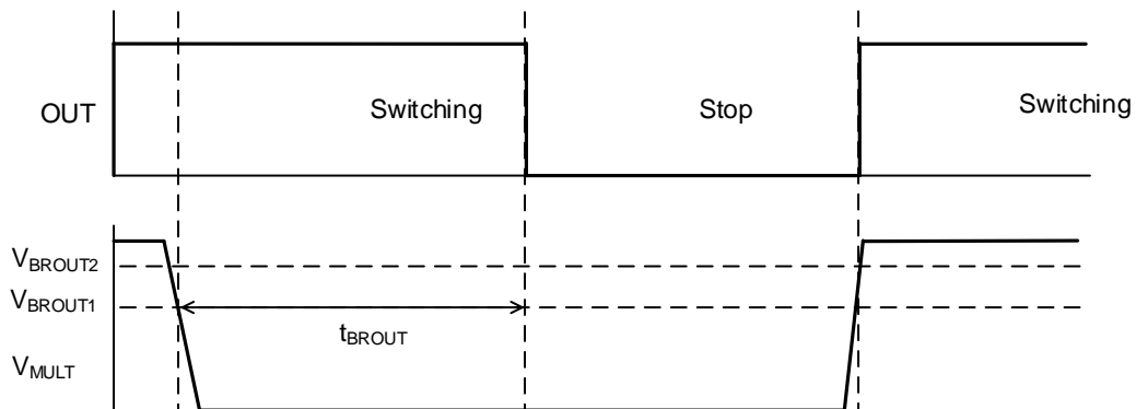
Figure 10. Brown Out
