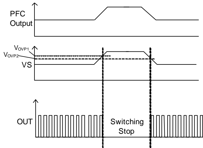
Figure 5. VS Overtoltage Protection Operation
