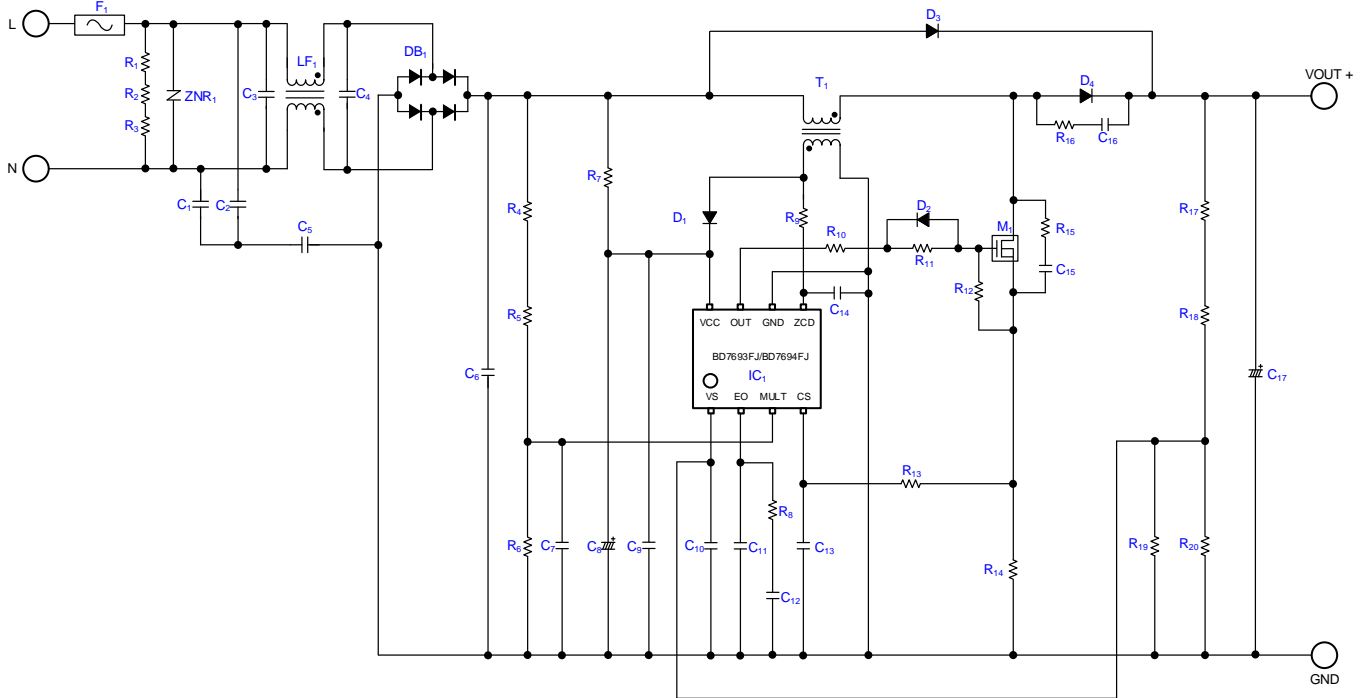
Figure 19. Application Example
