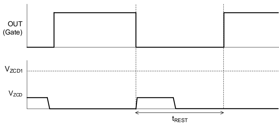
Figure 8. Restart Timer
