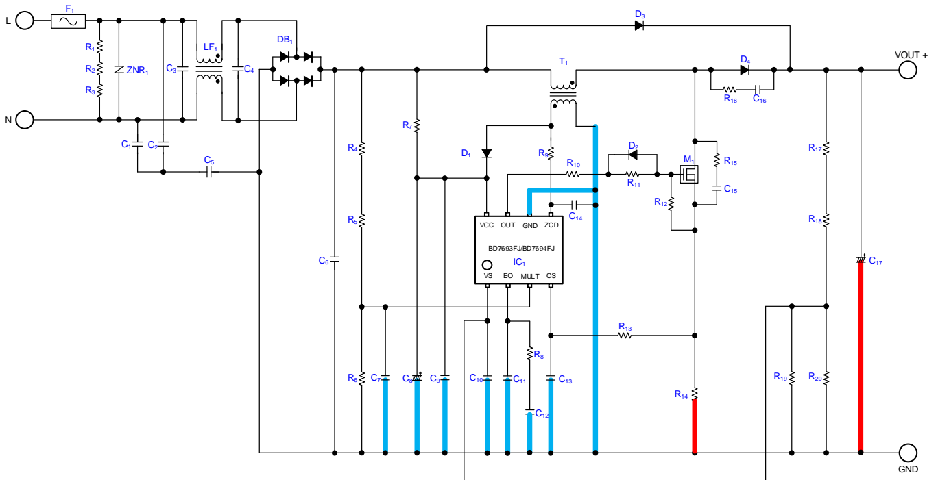
Figure 21. GND Line Layout
