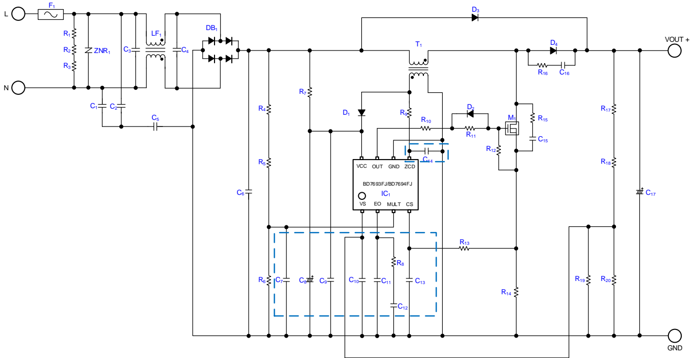
Figure 20. Parts Placement
