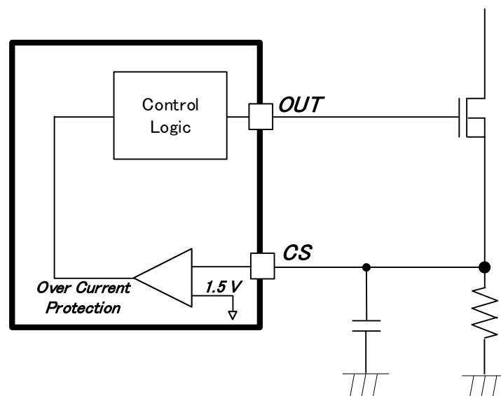
Figure 11. Current Limit
