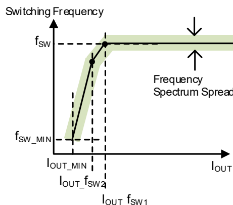
Figure 48. Switching Frequency
