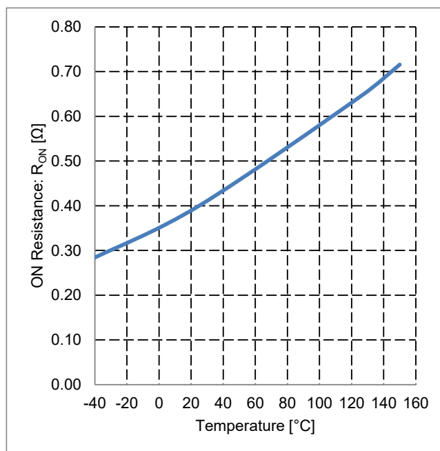
Figure 24. ON Resistance vs Temperature
