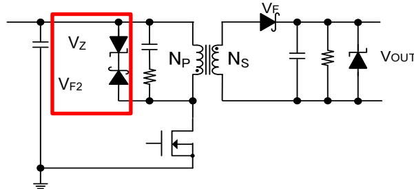
Figure 45. Snubber Circuit
