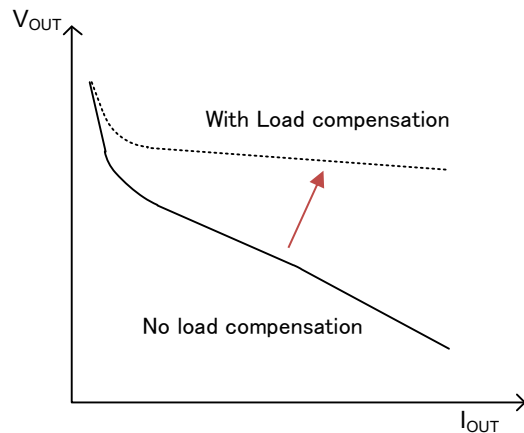
Figure 47. L_COMP Pin Voltage Compensation Example
