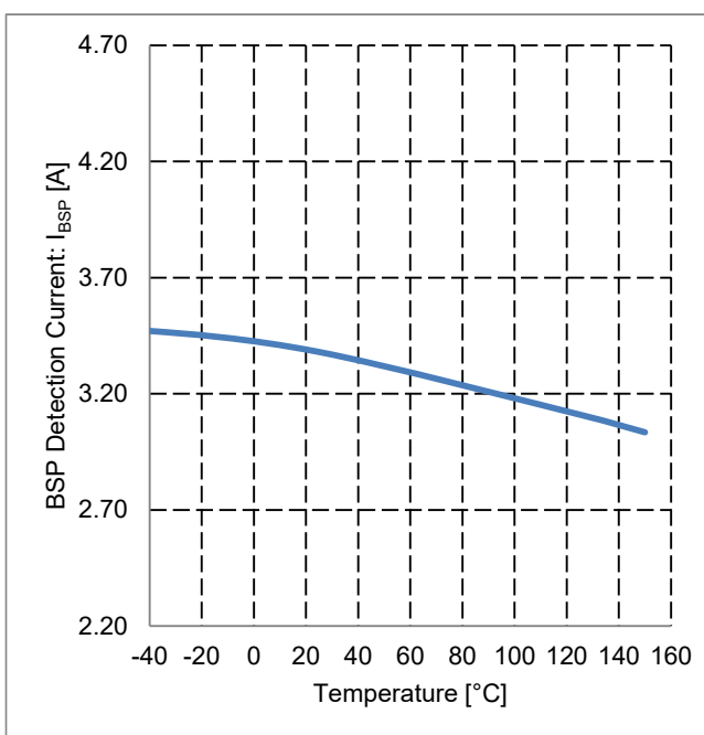
Figure 26. BSP Detection Current vs Temperature
