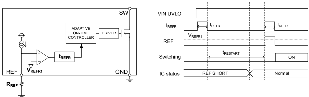
Figure 8. REFSHORT Protection Timing Chart
