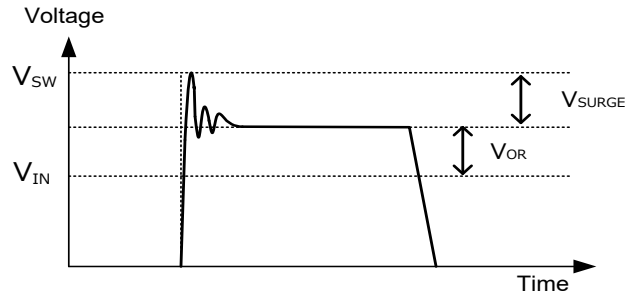
Figure 42. SW Waveform
