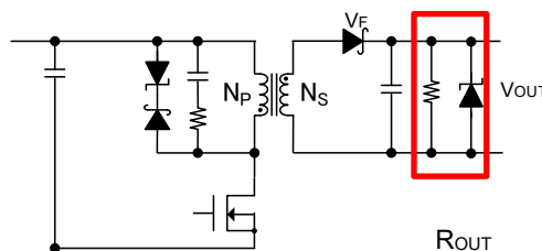
Figure 44. Zener Diode and Resistor to Secondary Output
