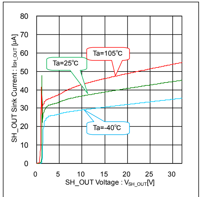
Figure 6. Circuit Current – SH_OUT Voltage (V SH_IN =0V)
