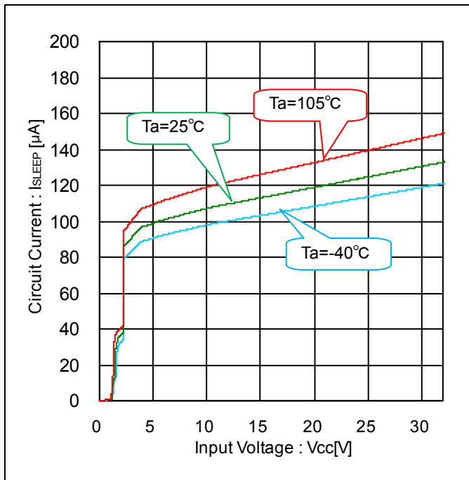
Figure 5. Circuit Current – Input Voltage (at Shut Down State)
