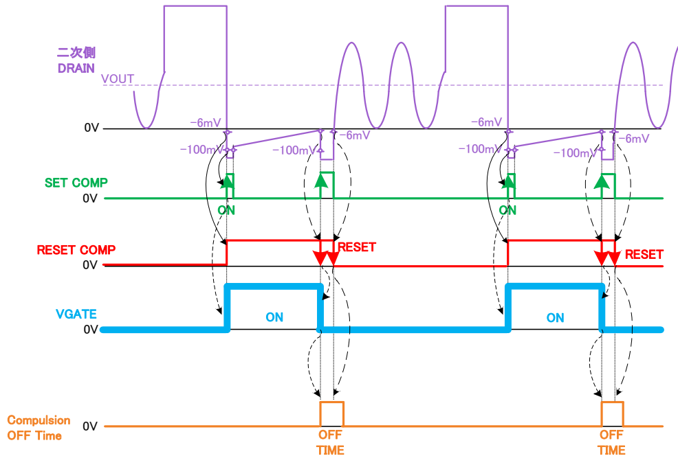
Figure 1. Operation sequence
