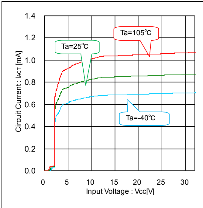
Figure 3. Circuit Current – Input Voltage (Stop Switching State)
