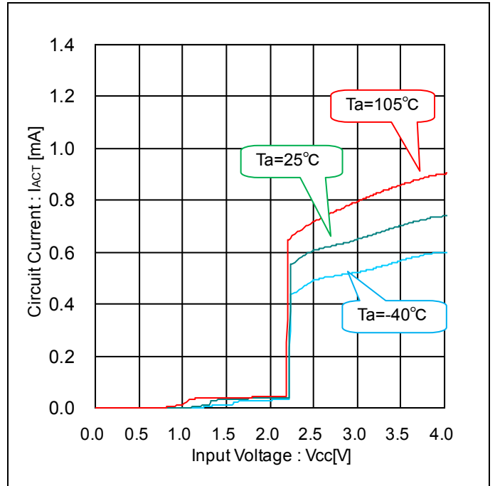
Figure 4. Circuit Current – Input Voltage (Stop Switching State V CC Zoom)
