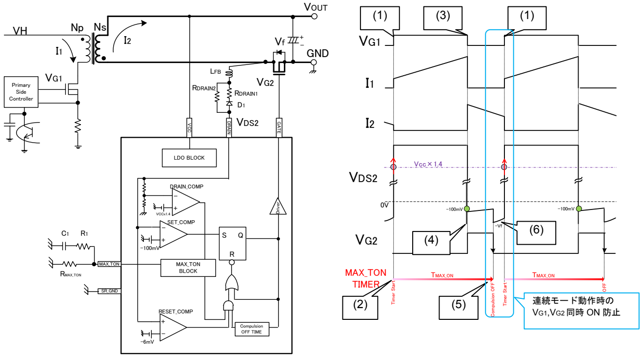
Figure 2. The drive sequence in continuous mode operation
