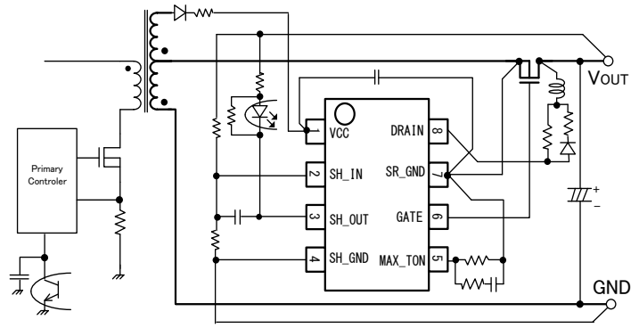
Flyback Application Circuit (High Side FET)
