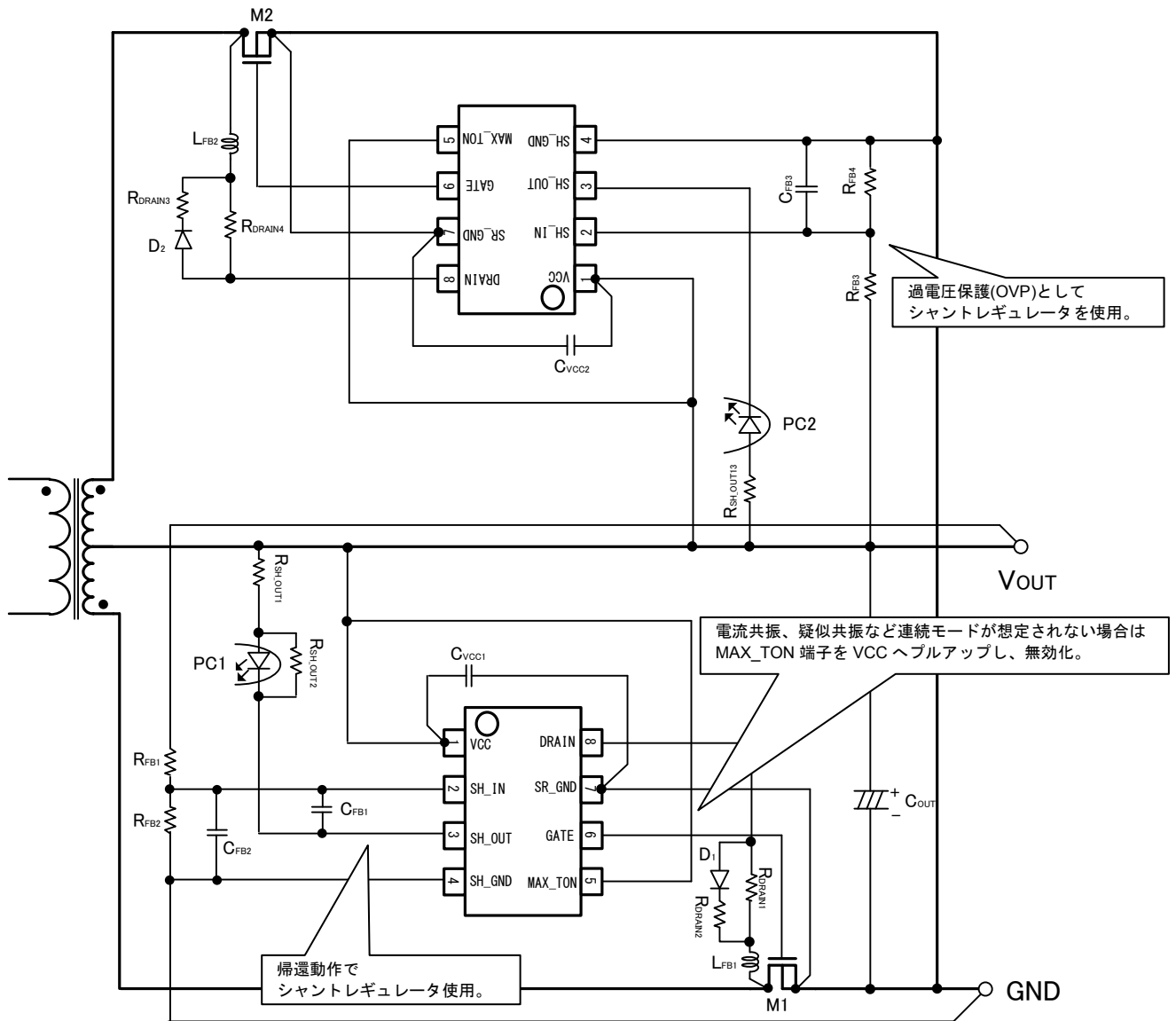
Figure 16. Resonant half-bridge application circuit
