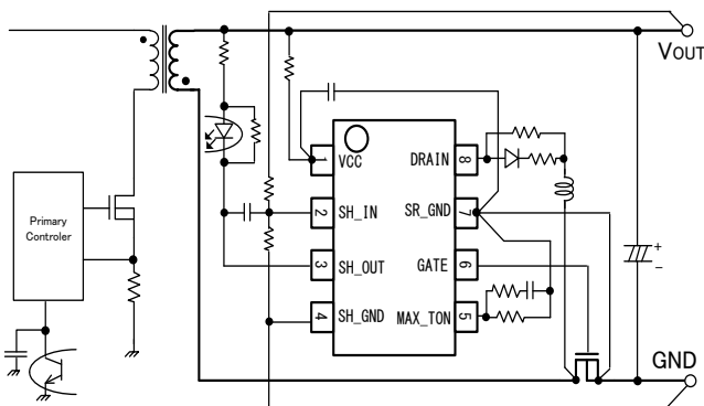
Flyback Application Circuit (Low Side FET)
