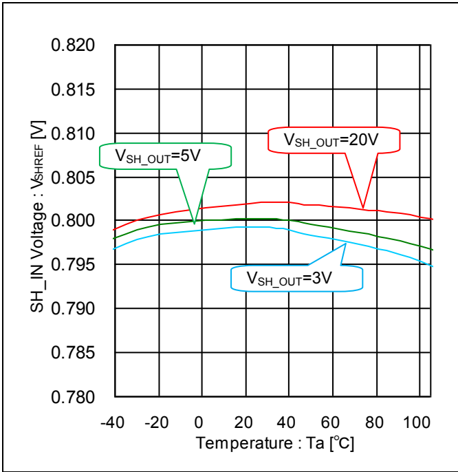
Figure 7. SH_IN Voltage vs Temperature (I SH_OUT =100uA)
