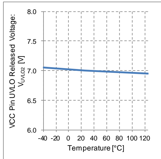
Figure 13. VCC Pin UVLO Released Voltage vs Temperature
