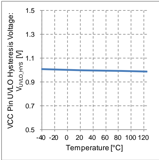
Figure 14. VCC Pin UVLO Hysteresis Voltage vs Temperature
