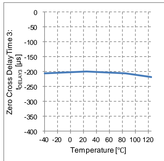
Figure 21. Zero Cross Delay Time 3 vs Temperature
