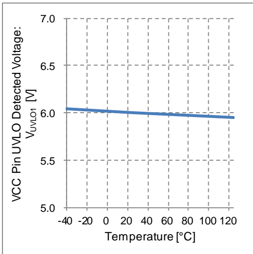
Figure 12. VCC Pin UVLO Detected Voltage vs Temperature
