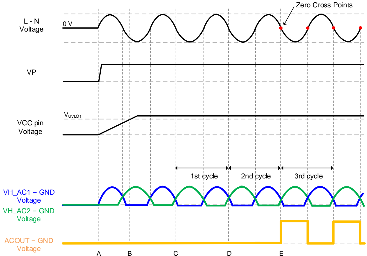
Figure 3. Startup Sequence
