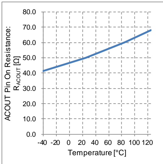
Figure 18. ACOUT Pin On Resistance vs Temperature
