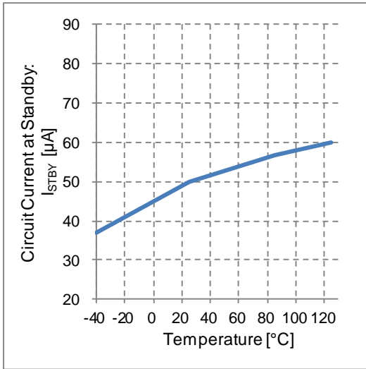
Figure 10. Circuit Current at Standby vs Temperature
