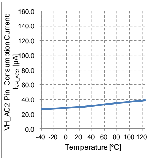
Figure 16. VH_AC2 Pin Consumption Current vs Temperature
