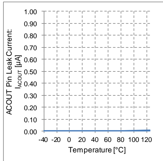
Figure 17. ACOUT Pin Leak Current vs Temperature
