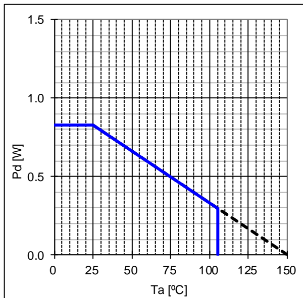
Figure 9. SOP-J7S Thermal Abatement Characteristic
