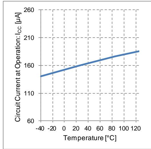
Figure 11. Circuit Current at Operation vs Temperature
