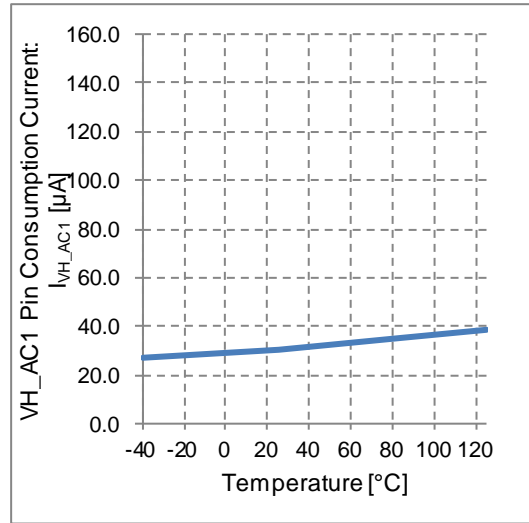
Figure 15. VH_AC1 Pin Consumption Current vs Temperature
