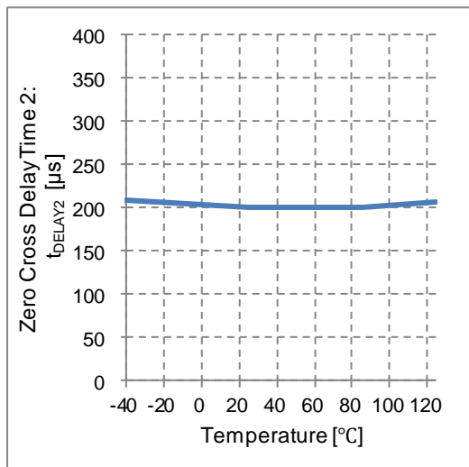
Figure 20. Zero Cross Delay Time 2 vs Temperature
