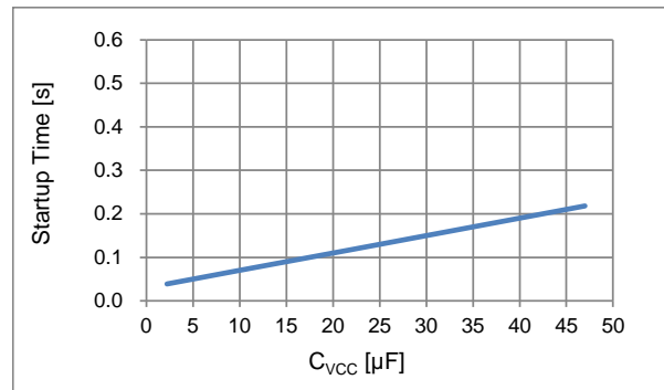
Figure 3. Startup Time vs C_{VCC}
