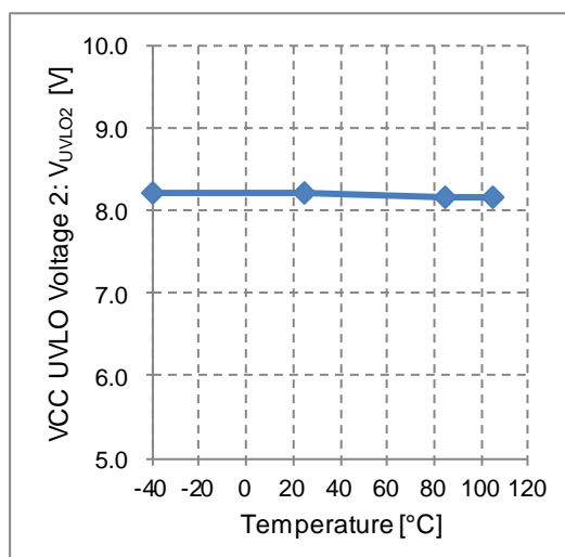
Figure 15. VCC UVLO Voltage 2 vs Temperature
