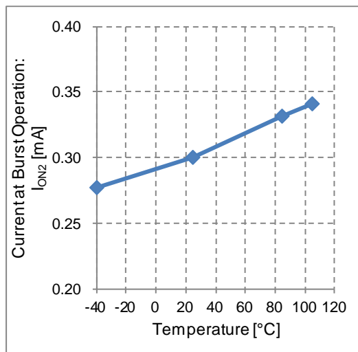
Figure 13. Current at Burst Operation vs Temperature
