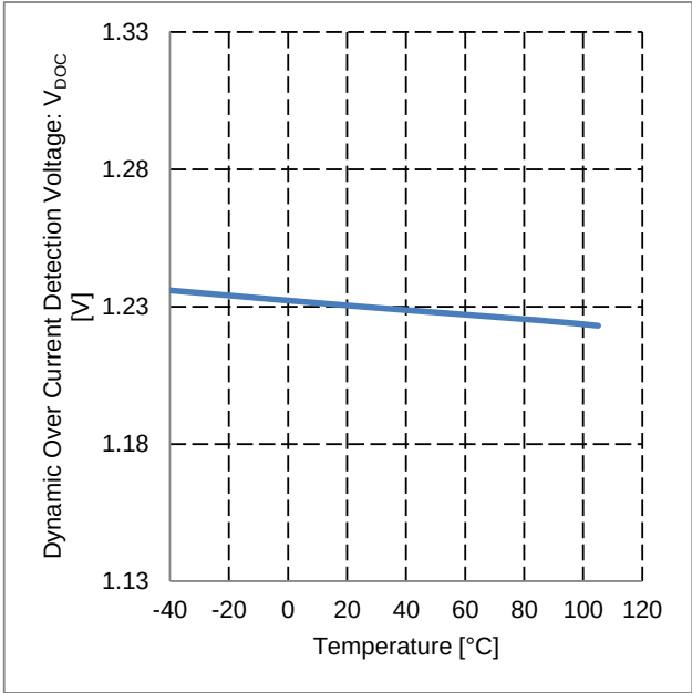
Figure 37. Dynamic Over Current Detection Voltage vs Temperature
