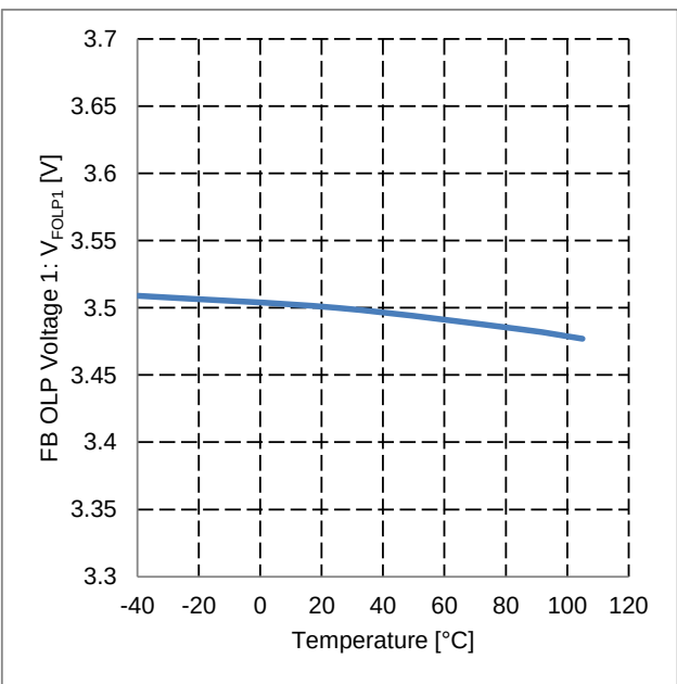
Figure 31. FB OLP Voltage 1 vs Temperature
