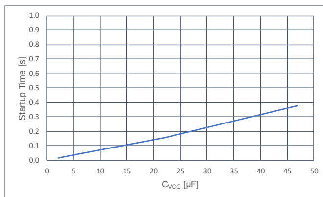
Figure 3. Startup Time vs C_{VCC}
