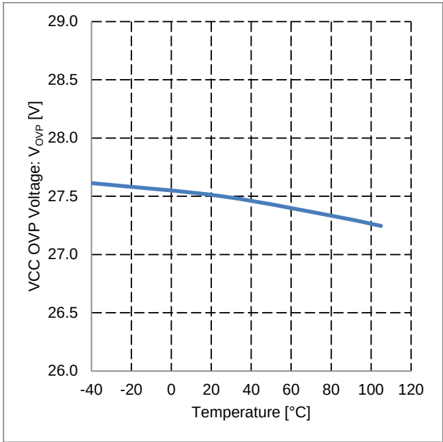
Figure 20. VCC OVP Voltage vs Temperature
