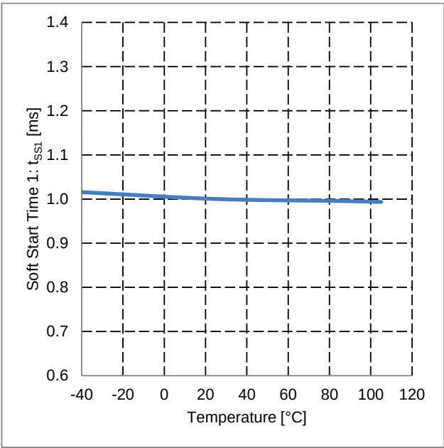
Figure 25. Soft Start Time 1 vs Temperature
