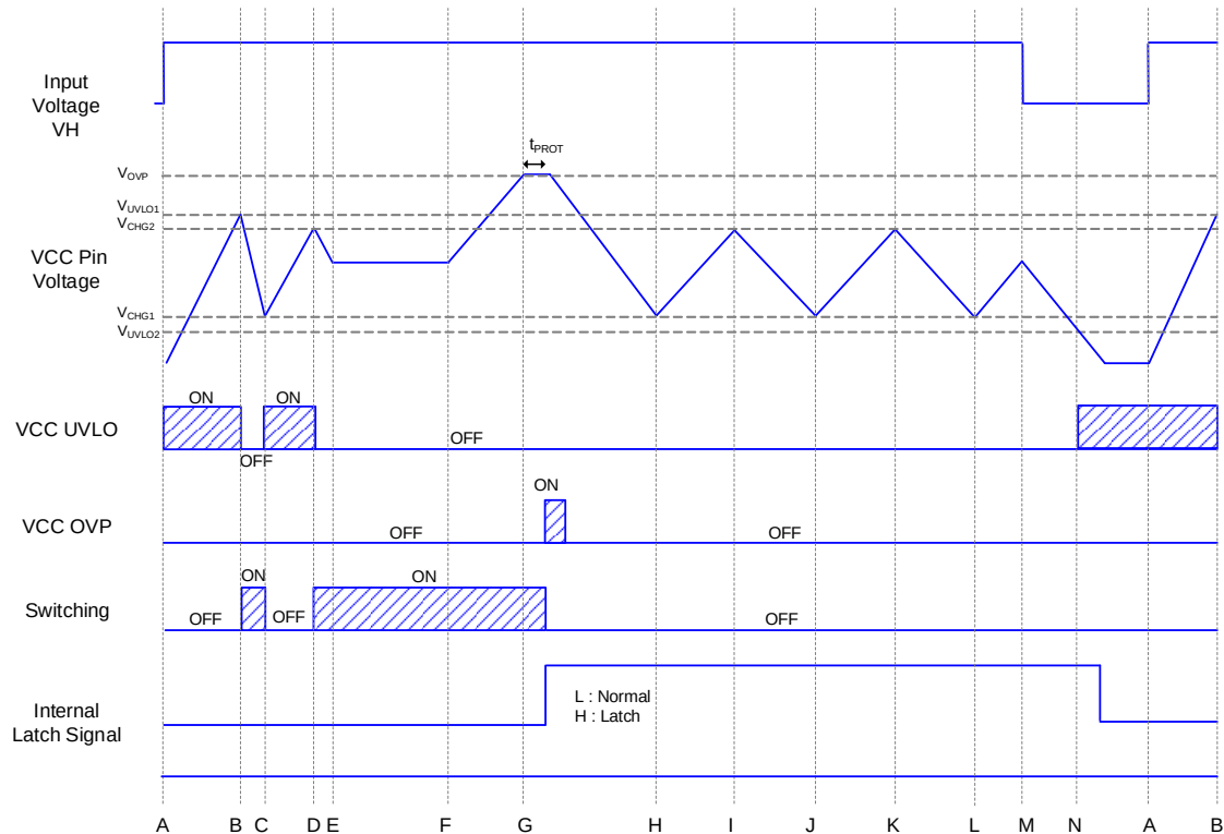
Figure 5. VCC UVLO / VCC OVP Timing Chart
