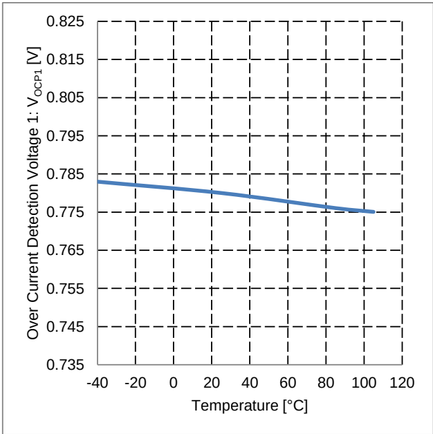
Figure 35. Over Current Detection Voltage 1 vs Temperature
