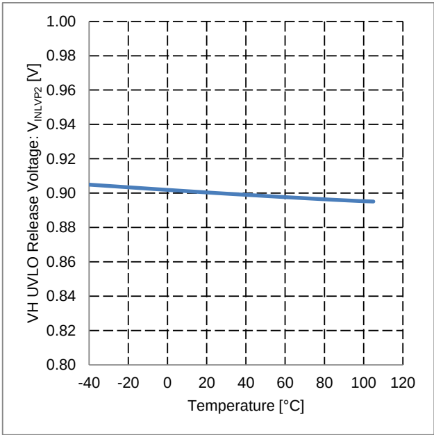
Figure 39. VH UVLO Release Voltage vs Temperature
