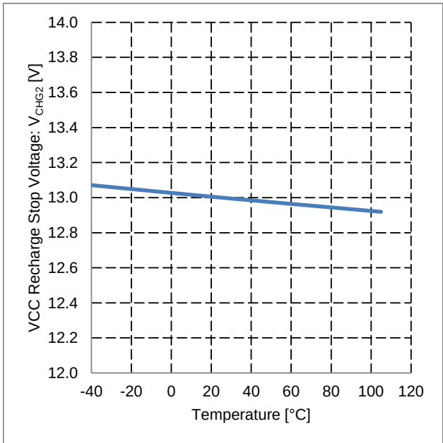
Figure 22. VCC Recharge Stop Voltage vs Temperature
