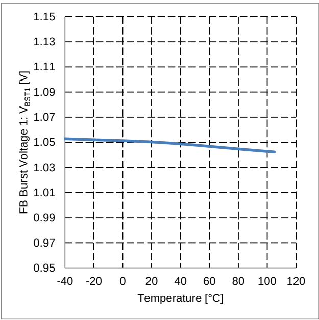
Figure 27. FB Burst Voltage 1 vs Temperature
