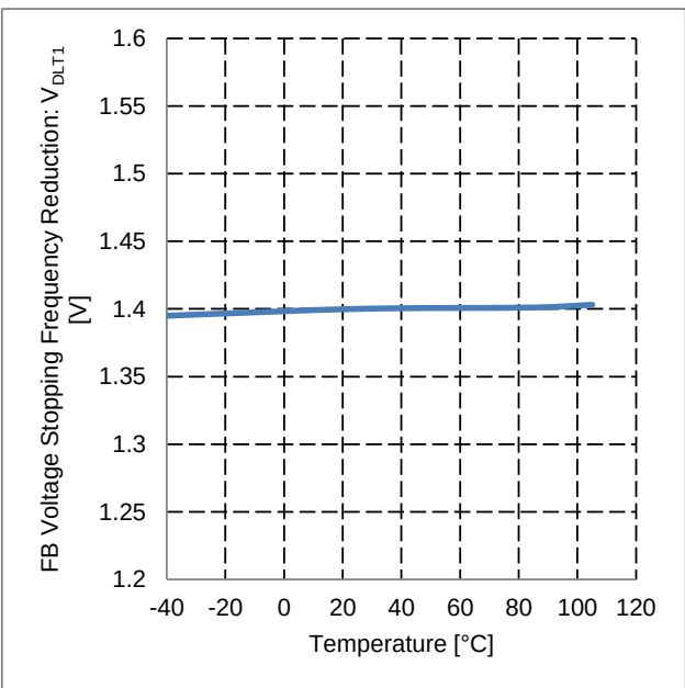
Figure 29. FB Voltage Stopping Frequency Reduction vs Temperature
