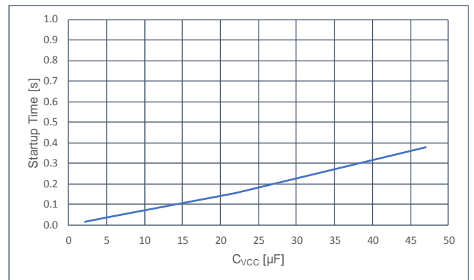
Figure 3. Startup Time vs C_{VCC}
