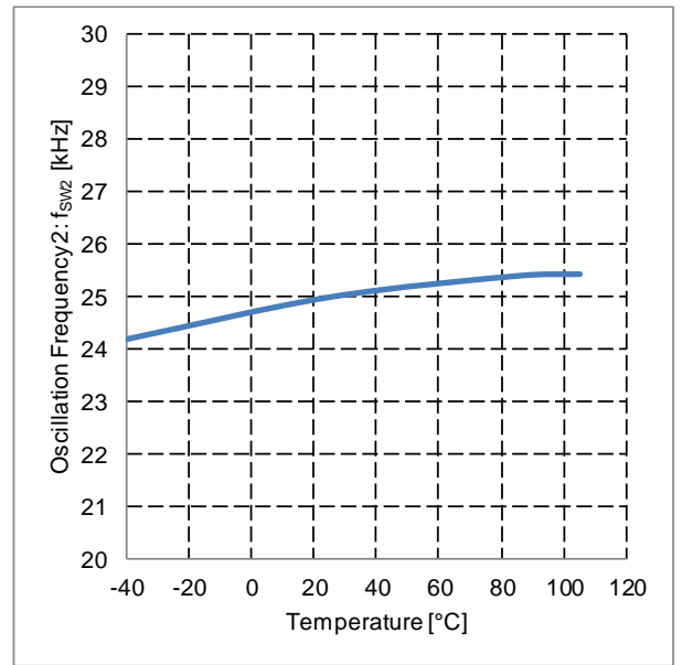
Figure 25. Oscillation Frequency 2 vs Temperature
