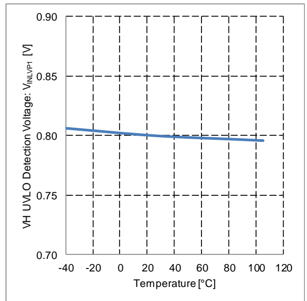
Figure 39. VH UVLO Detection Voltage vs Temperature
