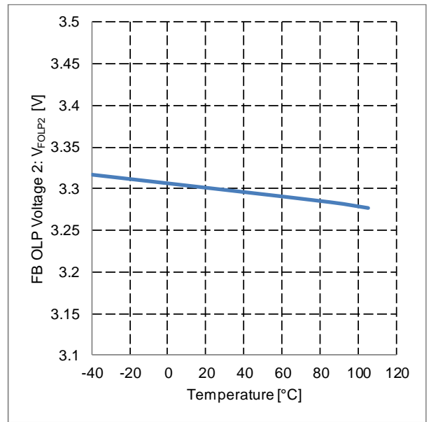
Figure 33. FB OLP Voltage 2 vs Temperature
