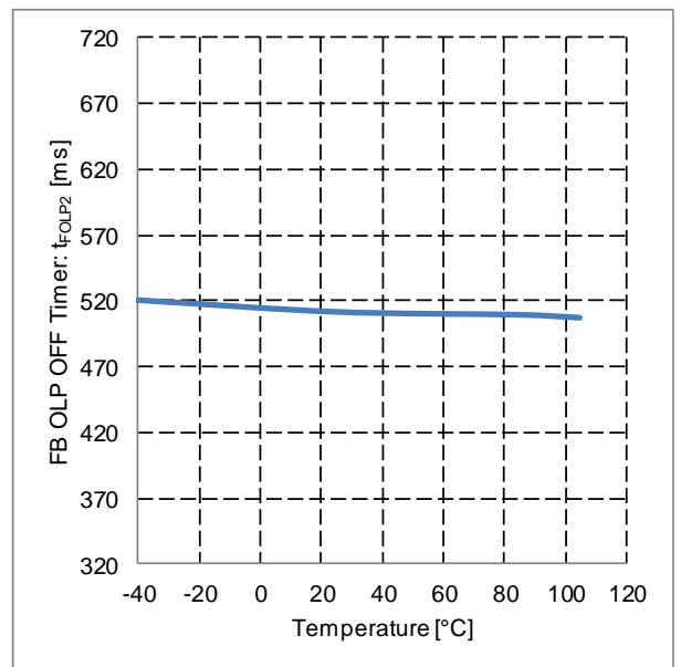
Figure 35. FB OLP OFF Timer vs Temperature
