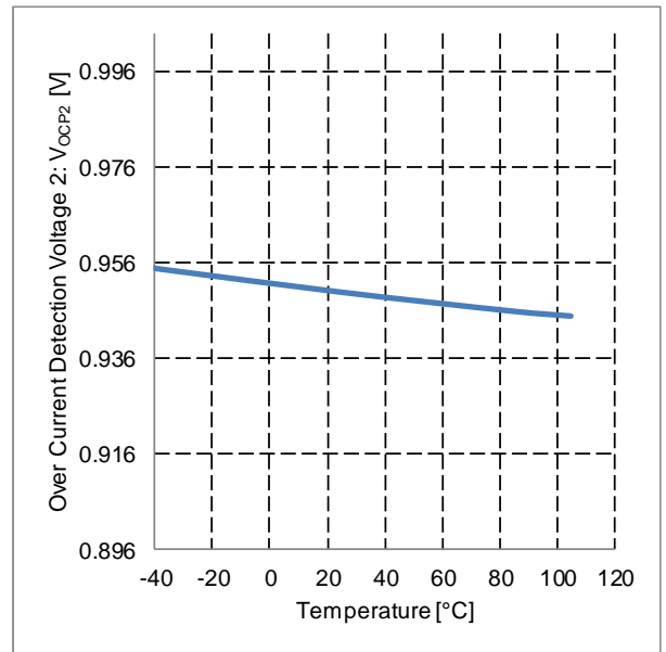
Figure 37. Over Current Detection Voltage 2 vs Temperature
