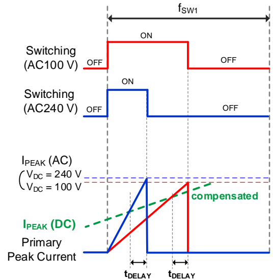
Figure 9. Built-in AC Compensation Voltage
