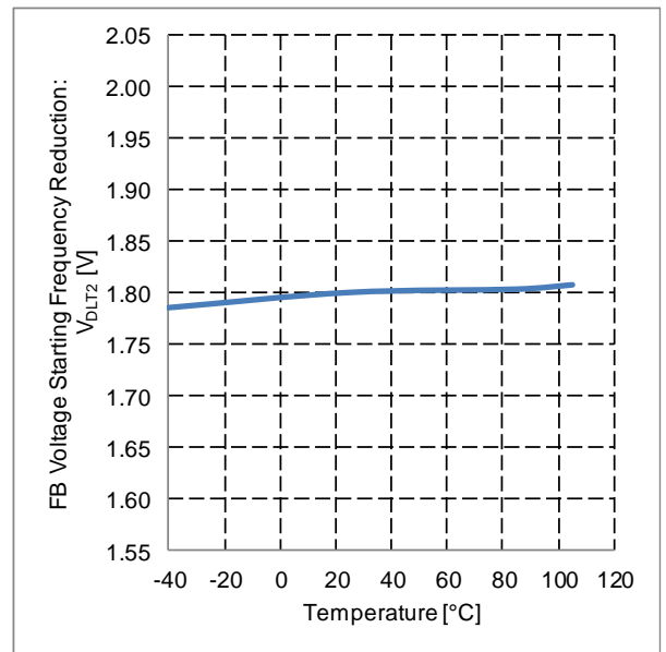
Figure 31. FB Voltage Starting Frequency Reduction vs Temperature
