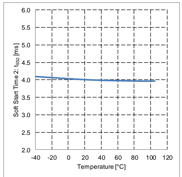
Figure 27. Soft Start Time 2 vs Temperature
