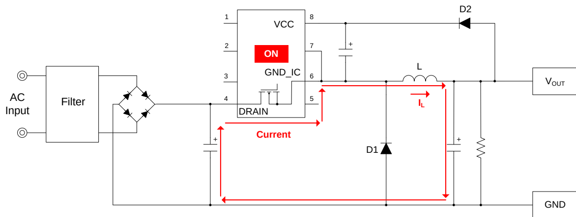
Figure 1. Buck Converter Operation (MOSFET = ON)
