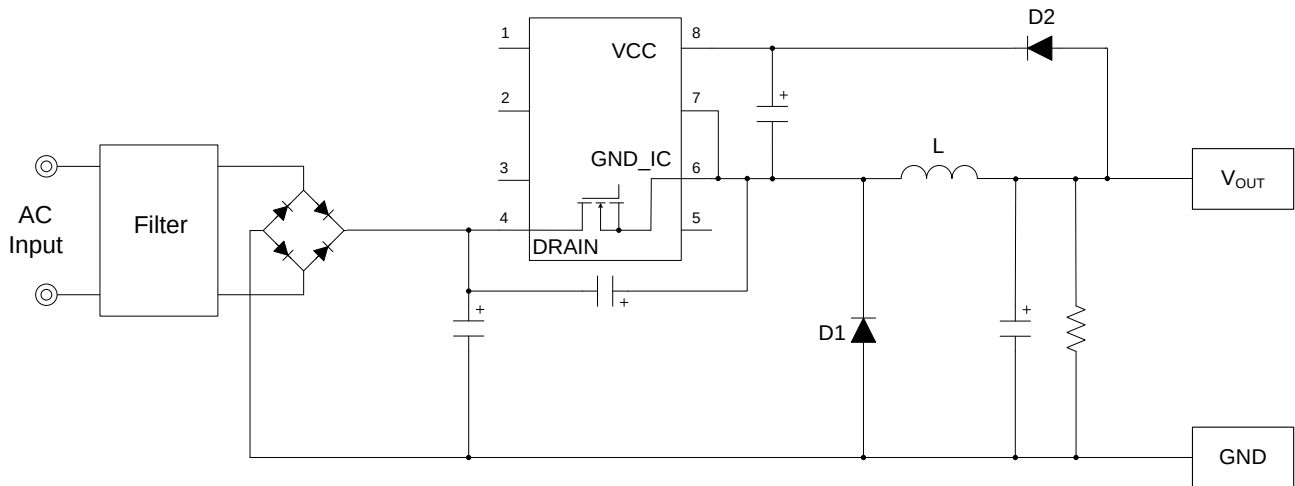
Figure 14. Application Circuit
