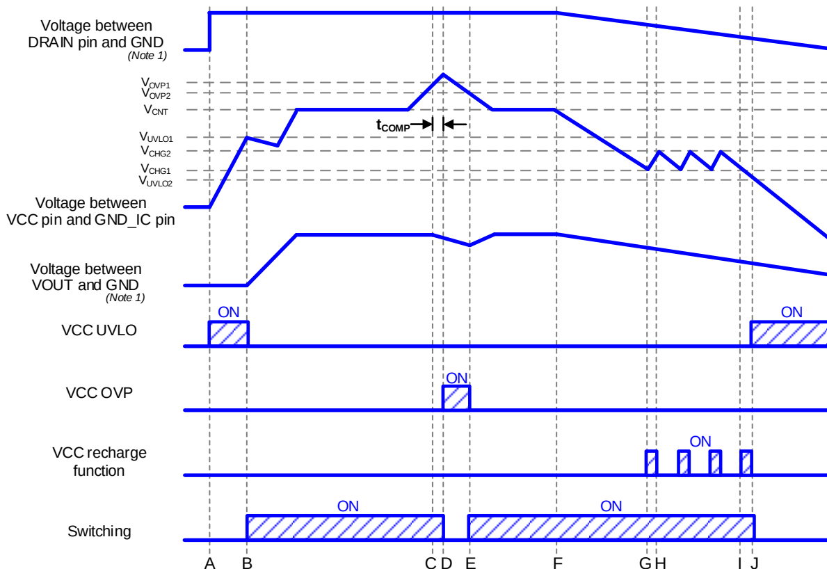
Figure 7. VCC UVLO / VCC OVP / VCC Recharge Function Timing Chart
