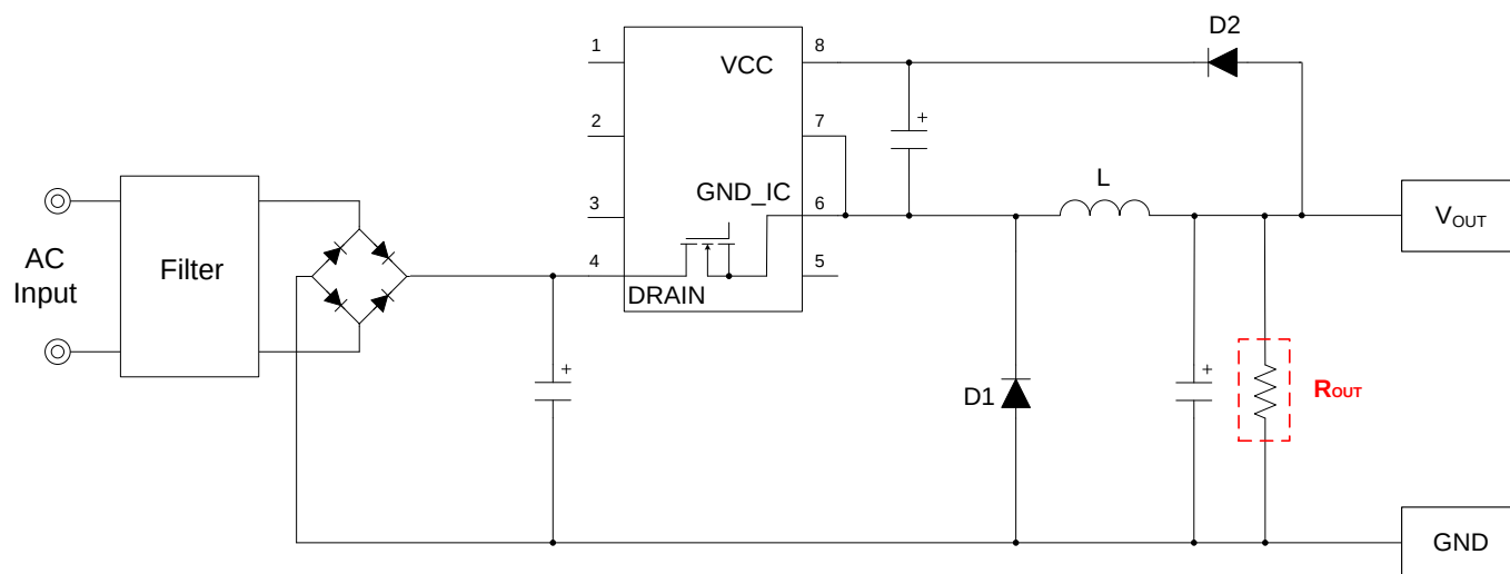
Figure 9. Location of Resistor R_{OUT}
