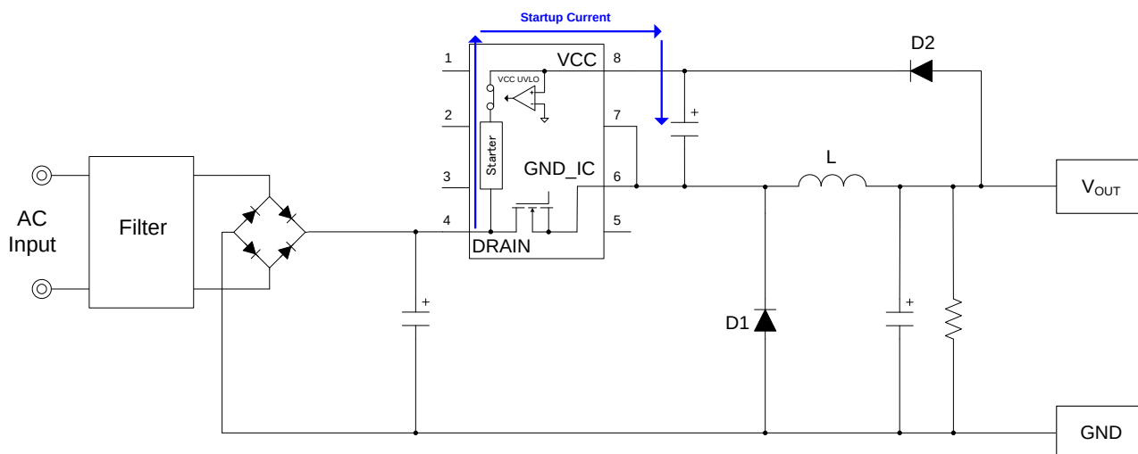
Figure 5. Startup Circuit
