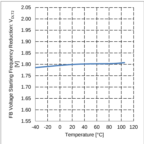
Figure 28. FB Voltage Starting Frequency Reduction vs Temperature
