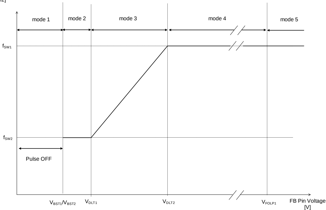
Figure 7. Switching Operation State Changes by FB Pin Voltage
