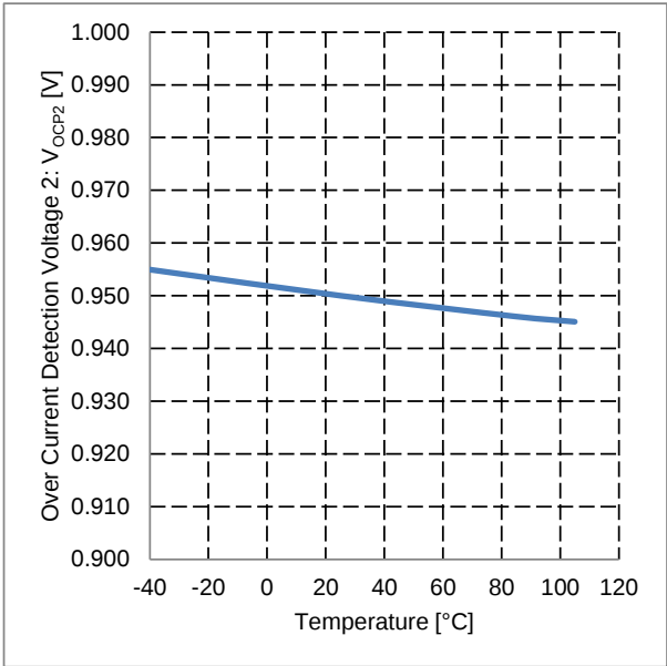
Figure 34. Over Current Detection Voltage 2 vs Temperature
