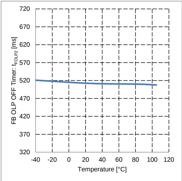
Figure 32. FB OLP OFF Timer vs Temperature
