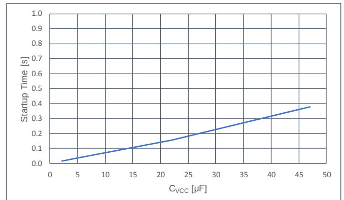
Figure 3. Startup Time vs C_{VCC}
