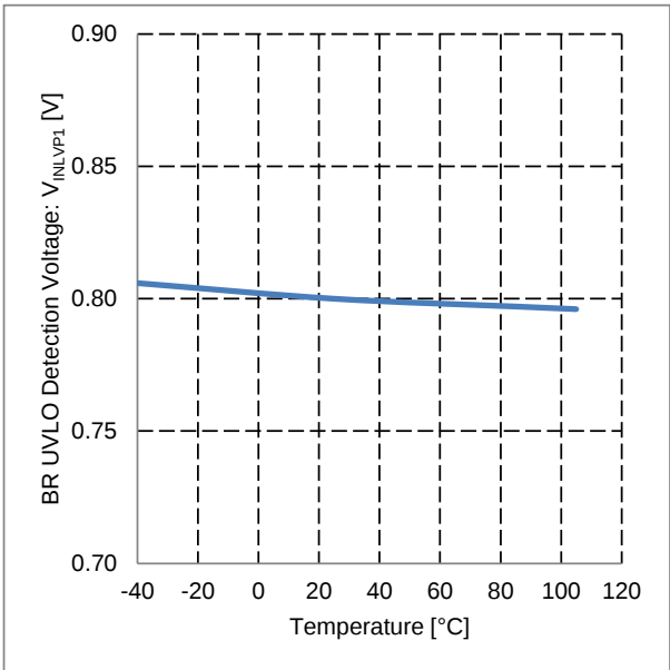
Figure 36. BR UVLO Detection Voltage vs Temperature
