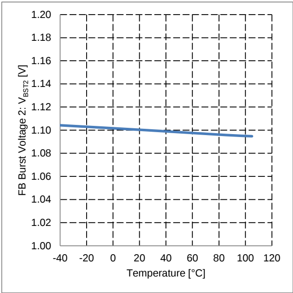
Figure 26. FB Burst Voltage 2 vs Temperature
