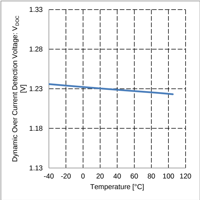
Figure 43. Dynamic Over Current Detection Voltage vs Temperature
