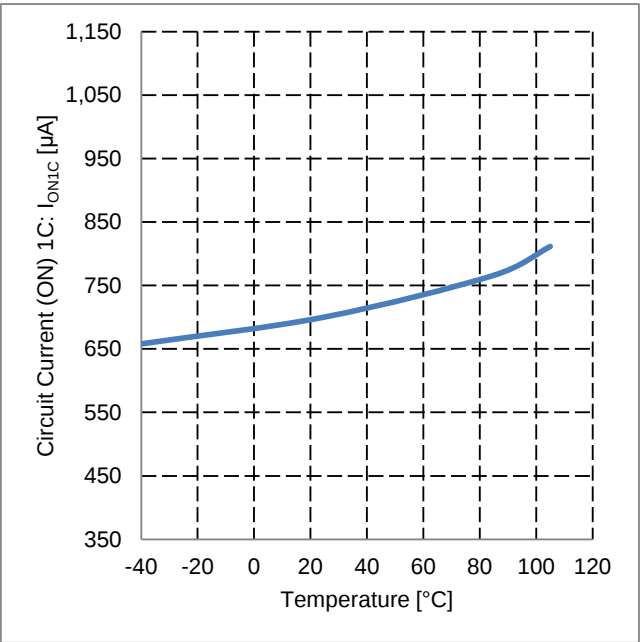
Figure 17. Circuit Current (ON) 1C vs Temperature
