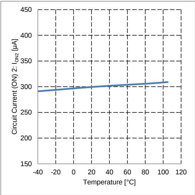
Figure 18. Circuit Current (ON) 2 vs Temperature
