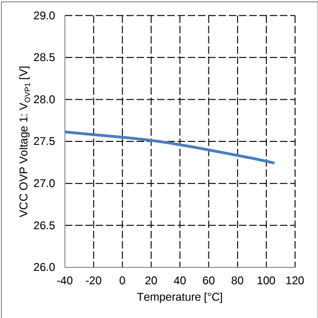
Figure 21. VCC OVP Voltage 1 vs Temperature
