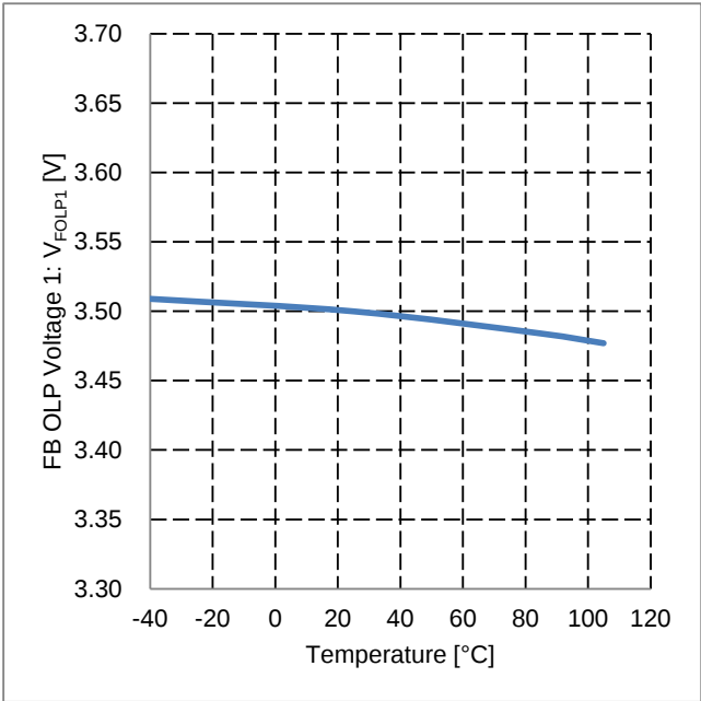
Figure 37. FB OLP Voltage 1 vs Temperature
