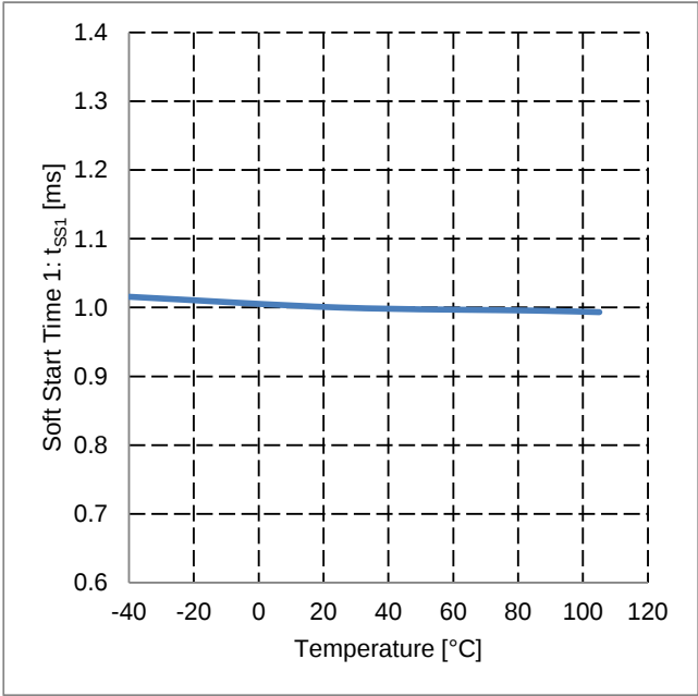
Figure 29. Soft Start Time 1 vs Temperature
