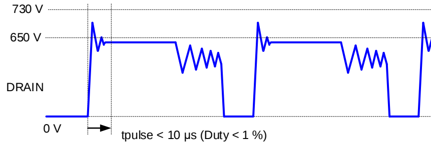
Figure 14. DRAIN pin Ringing Waveform
