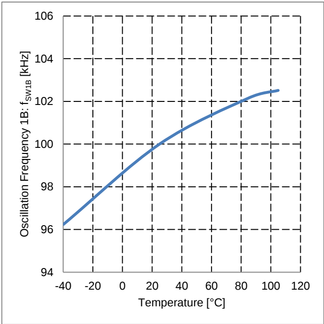
Figure 26. Oscillation Frequency 1B vs Temperature
