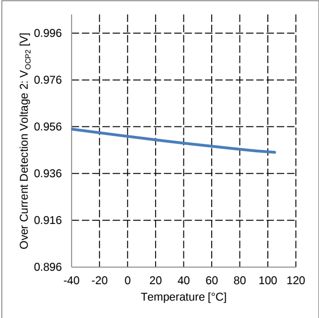
Figure 42. Over Current Detection Voltage 2 vs Temperature
