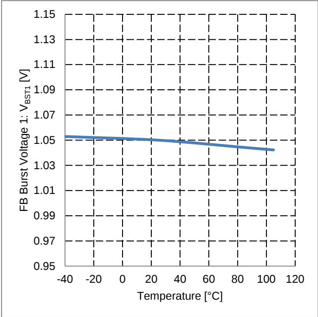
Figure 31. FB Burst Voltage 1 vs Temperature
