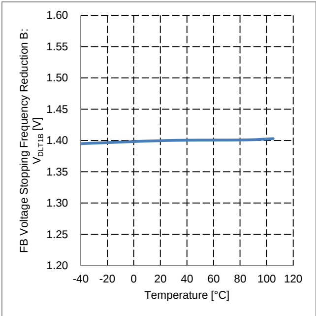
Figure 34. FB Voltage Stopping Frequency Reduction B vs Temperature
