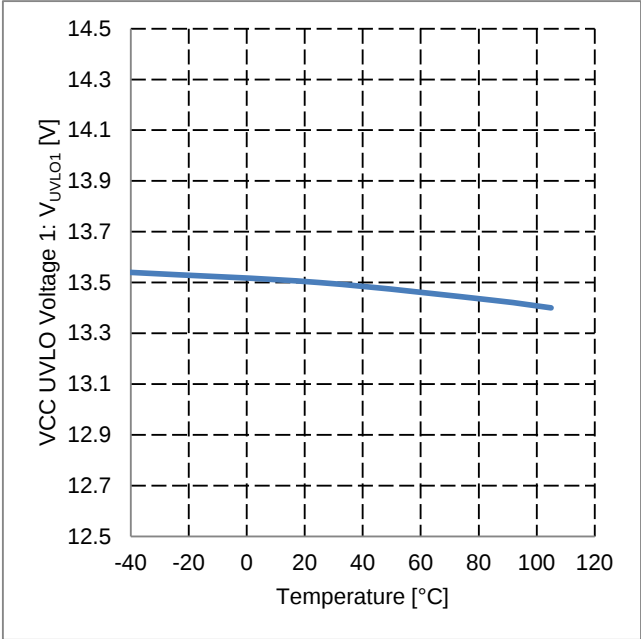
Figure 19. VCC UVLO Voltage 1 vs Temperature
