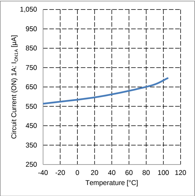
Figure 15. Circuit Current (ON) 1A vs Temperature
