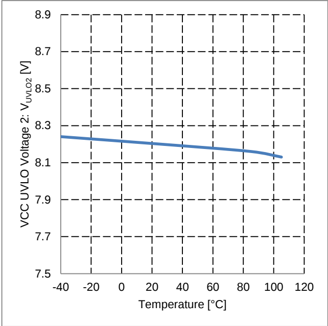
Figure 20. VCC UVLO Voltage 2 vs Temperature
