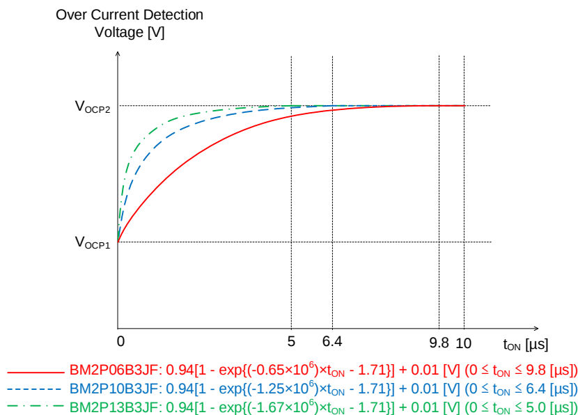
Figure 10. Over Current Detection Voltage
