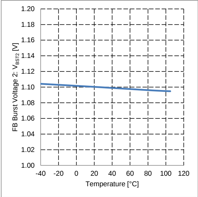
Figure 32. FB Burst Voltage 2 vs Temperature
