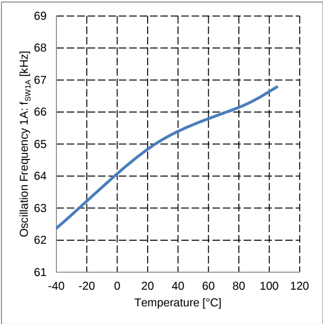
Figure 25. Oscillation Frequency 1A vs Temperature
