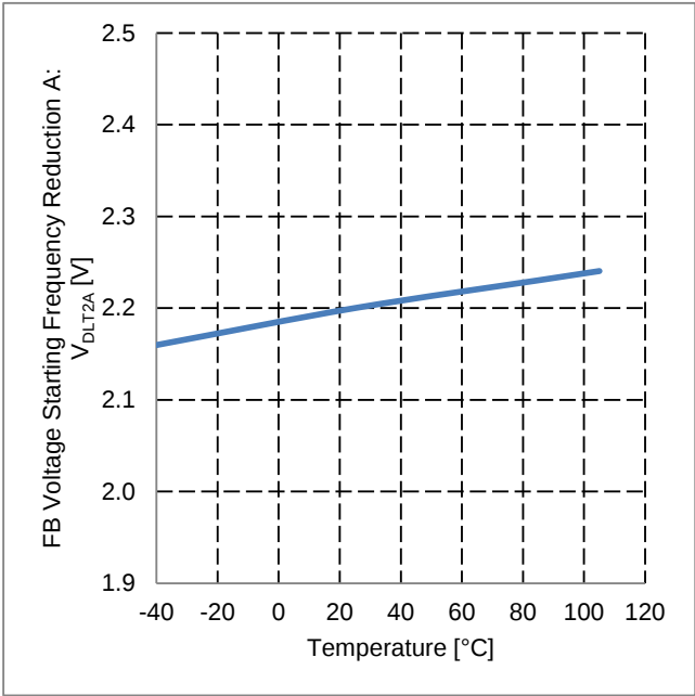
Figure 35. FB Voltage Starting Frequency Reduction A vs Temperature
