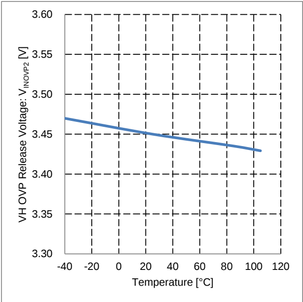
Figure 47. V H OVP Release Voltage vs Temperature
