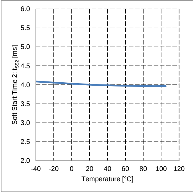
Figure 30. Soft Start Time 2 vs Temperature
