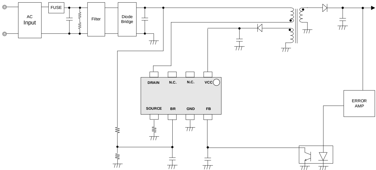
Figure 13. Flyback Application Diagram
