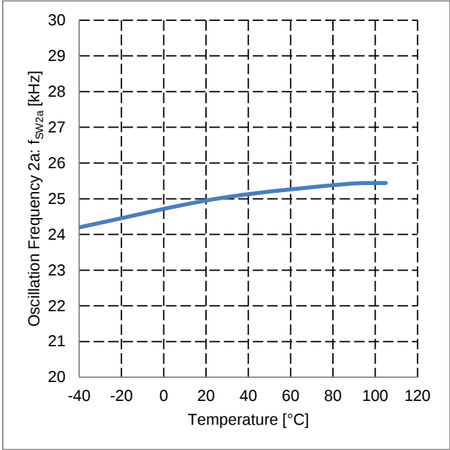
Figure 28. Oscillation Frequency 2a vs Temperature
