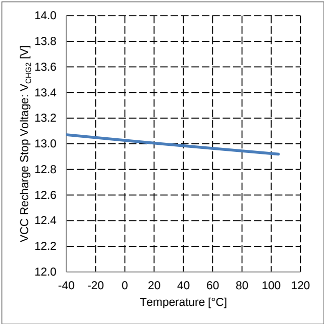
Figure 24. VCC Recharge Stop Voltage vs Temperature
