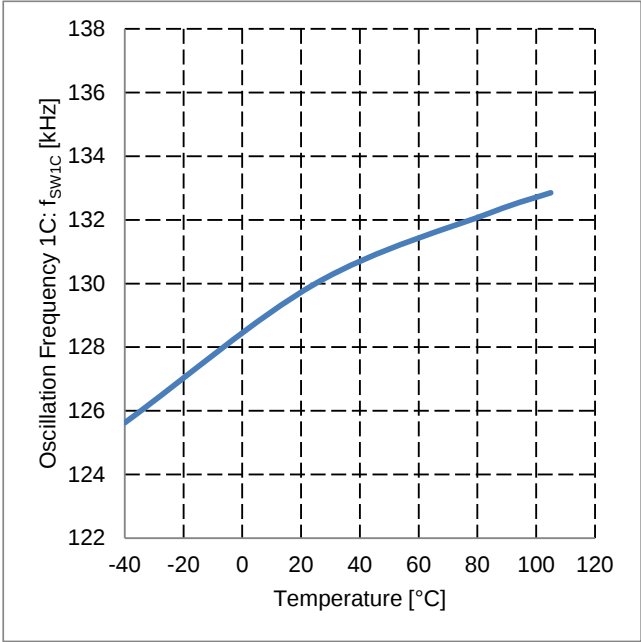
Figure 27. Oscillation Frequency 1C vs Temperature
