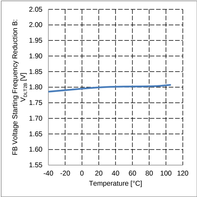
Figure 36. FB Voltage Starting Frequency Reduction B vs Temperature
