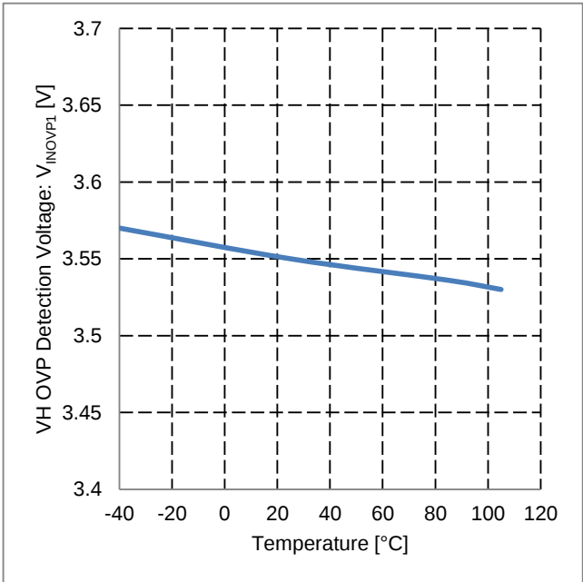
Figure 46. VH OVP Detection Voltage vs Temperature
