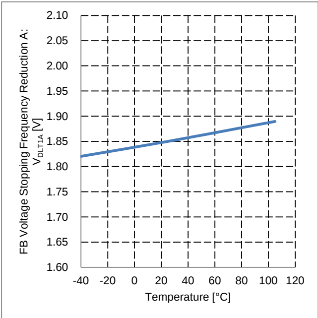
Figure 33. FB Voltage Stopping Frequency Reduction A vs Temperature
