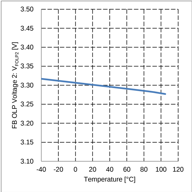
Figure 38. FB OLP Voltage 2 vs Temperature
