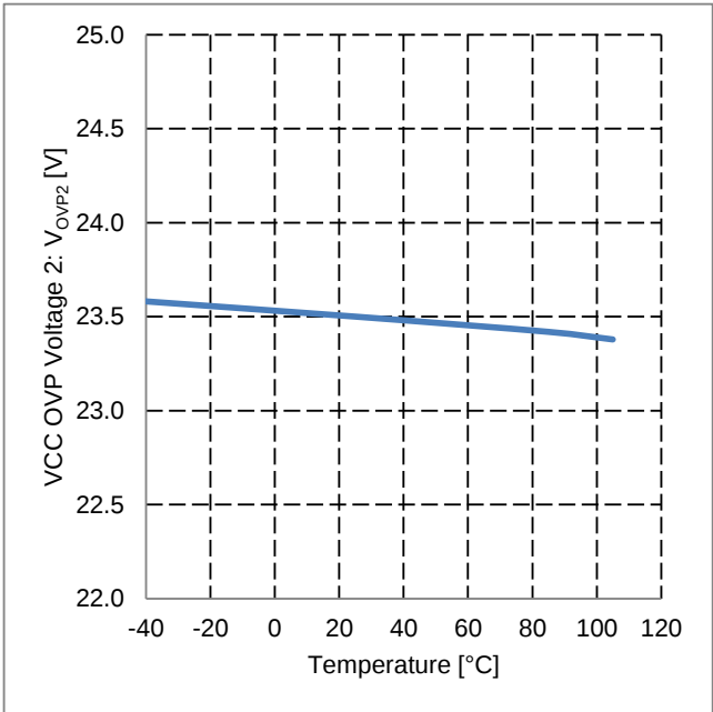
Figure 22. VCC OVP Voltage 2 vs Temperature
