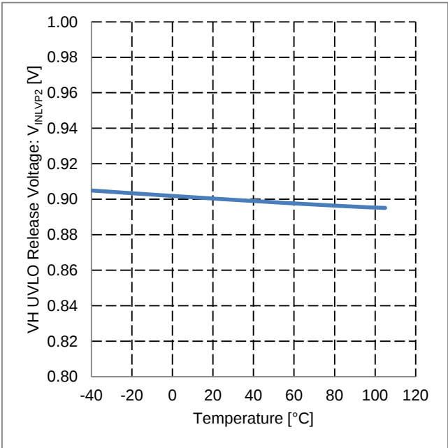
Figure 45. VH UVLO Release Voltage vs Temperature
