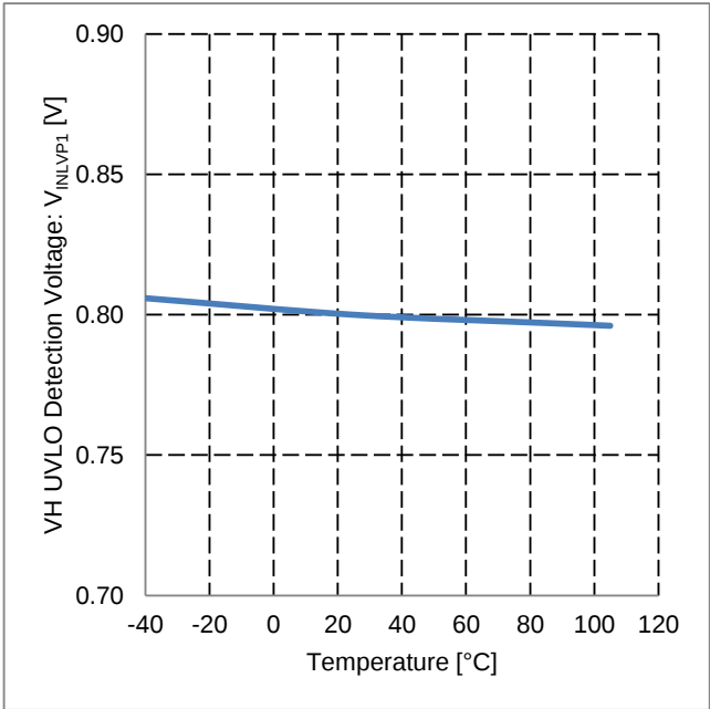
Figure 44. VH UVLO Detection Voltage vs Temperature
