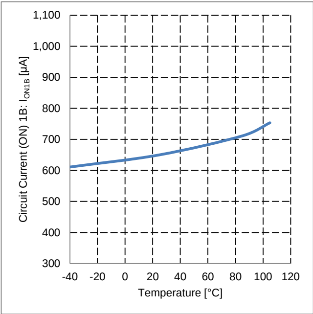
Figure 16. Circuit Current (ON) 1B vs Temperature
