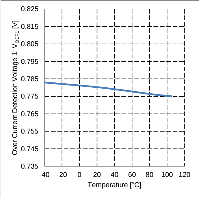
Figure 41. Over Current Detection Voltage 1 vs Temperature
