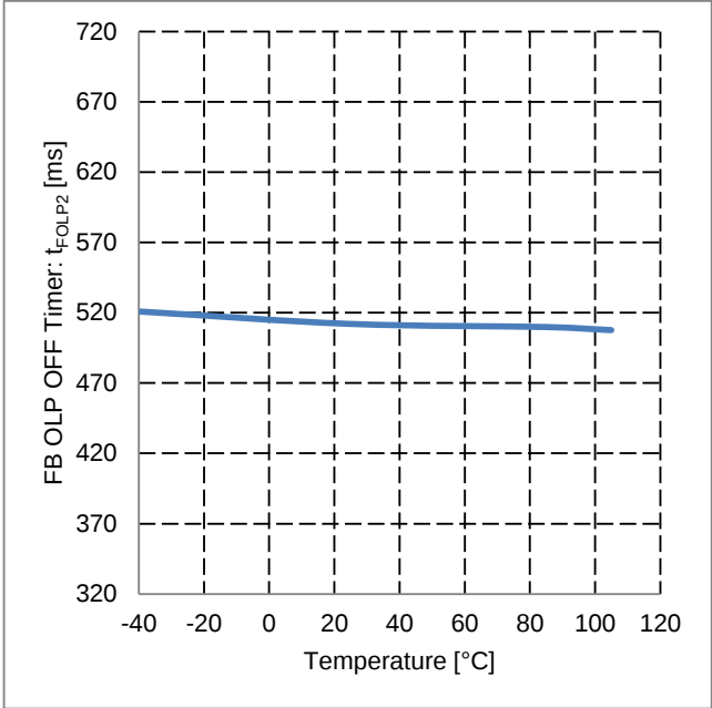
Figure 40. FB OLP OFF Timer vs Temperature
