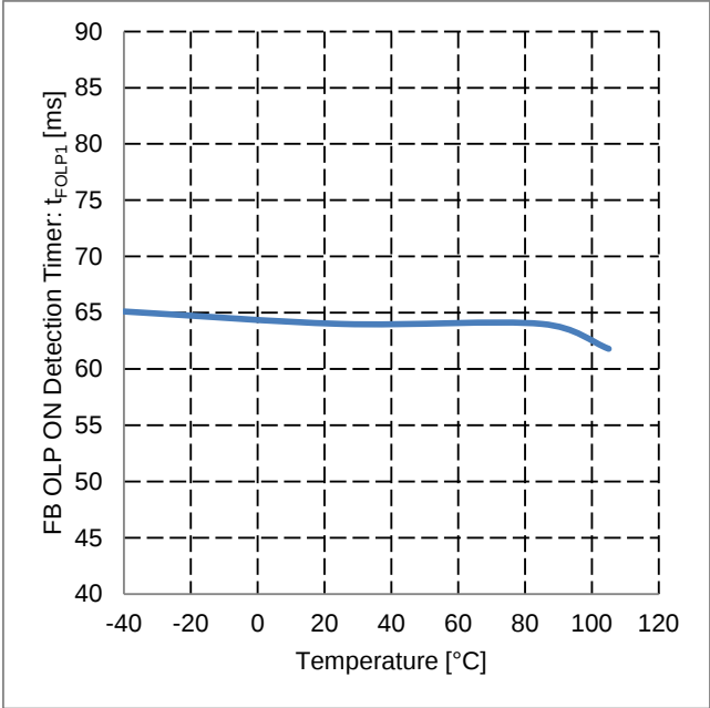
Figure 39. FB OLP ON Detection Timer vs Temperature
