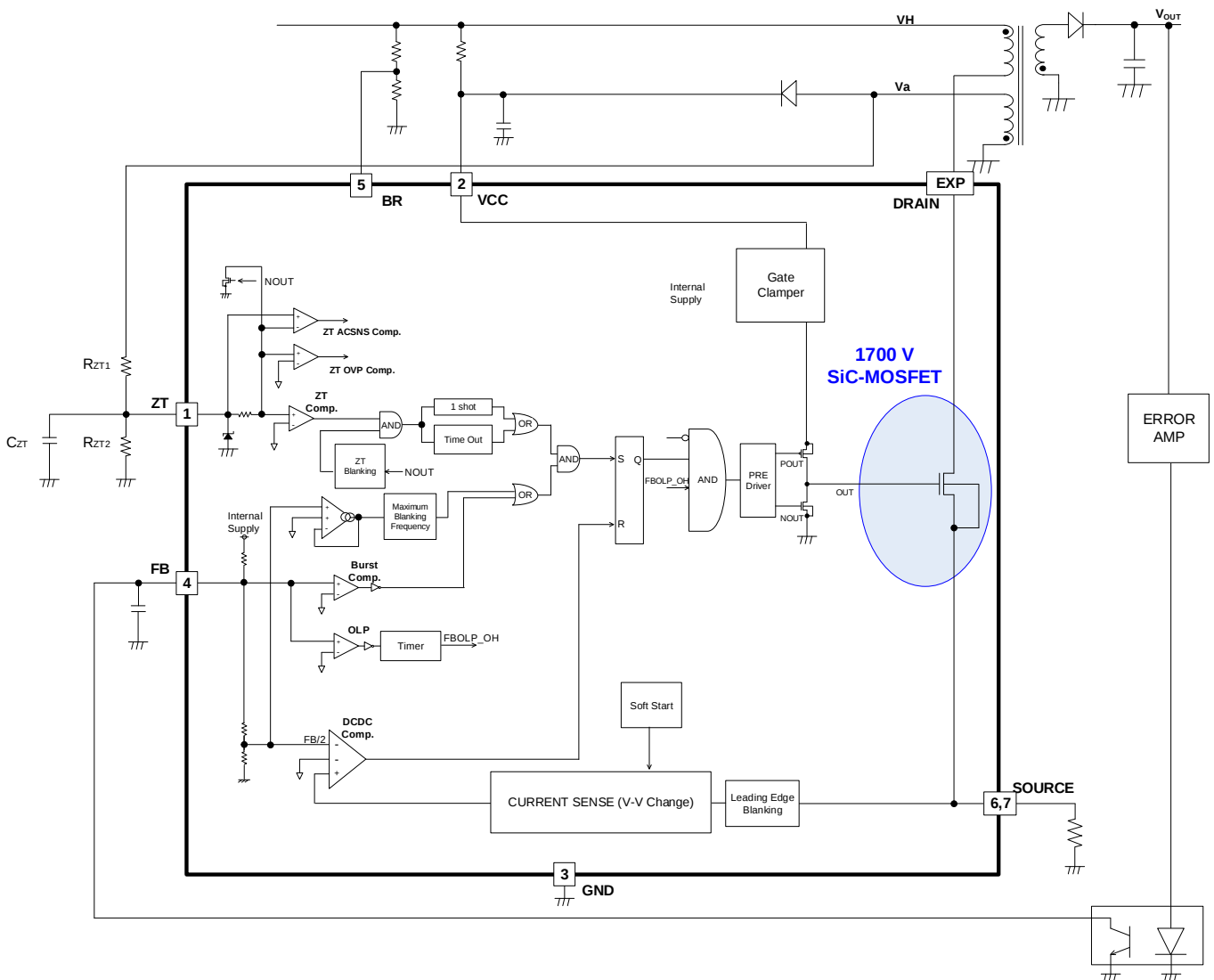
Figure 5. Block Diagram of SOURCE Switching Current
