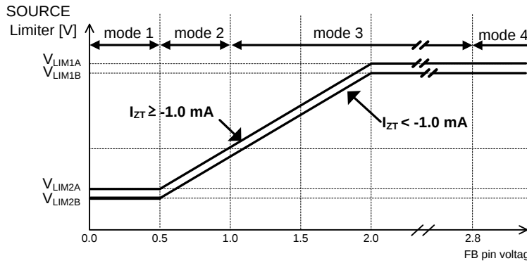
Figure 6. SOURCE Switching: SOURCE Limiter vs FB Pin Voltage
