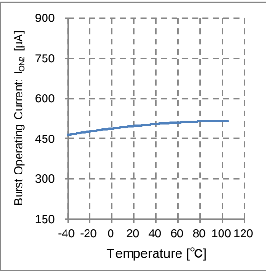
Figure 18. Burst Operating Current vs Temperature
