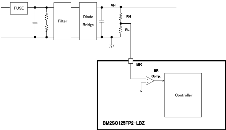
Figure 15. BR UVLO Function
