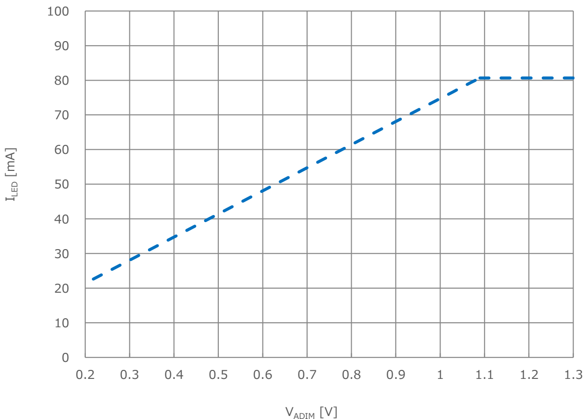
Figure 12. I_{LED} VS V_{ADIM}
