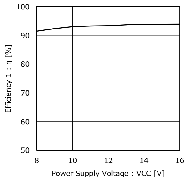
Figure 9. Efficiency 1 vs Power Supply Voltage ( R_{RT} = 33.3\text{ k}\Omega , R_{SET} = 15.1\text{ k}\Omega , LED 直列数 = 10, LED 並列数 = 4)
