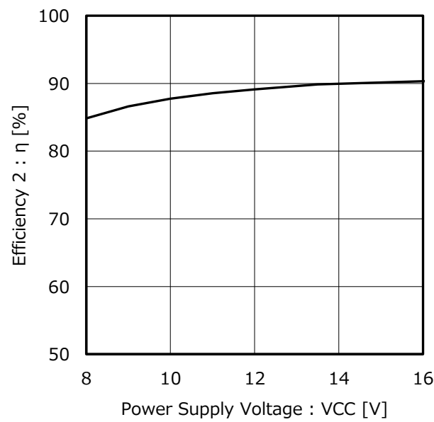
Figure 10. Efficiency 2 vs Power Supply Voltage ( R_{RT} = 3.8\text{ k}\Omega , R_{SET} = 15.1\text{ k}\Omega , LED 直列数 = 10, LED 並列数 = 4)
