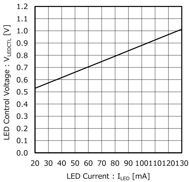
Figure 7. LED Control Voltage vs LED Current
