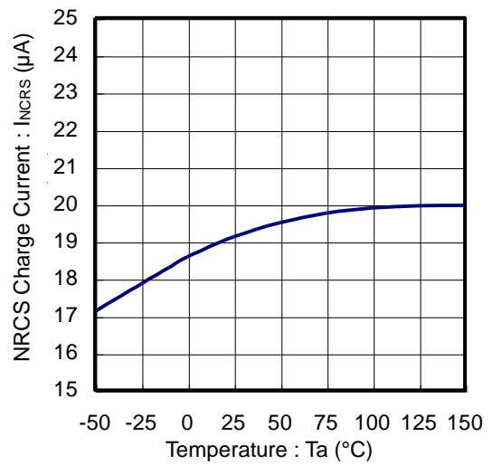
Figure 22. NRCS Charge Current vs Temperature
