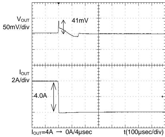
Figure 5. Transient Response (4A → 0A) C_{OUT}=100\mu F
