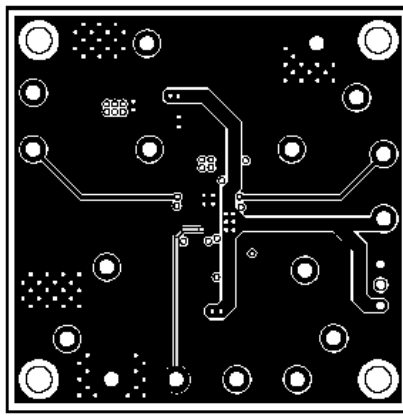
Middle Layer_2
