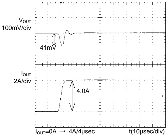
Figure 3. Transient Response (0A → 4A) C_{OUT}=47\mu F, C_{FB}=0.01\mu F
