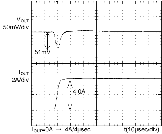
Figure 2. Transient Response (0A → 4A) C_{OUT}=100\mu F
