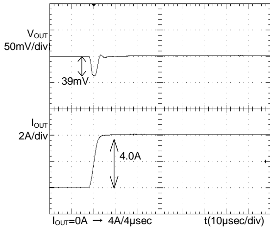
Figure 1. Transient Response (0A → 4A) C_{OUT}=22\mu F, C_{FB}=0.01\mu F
