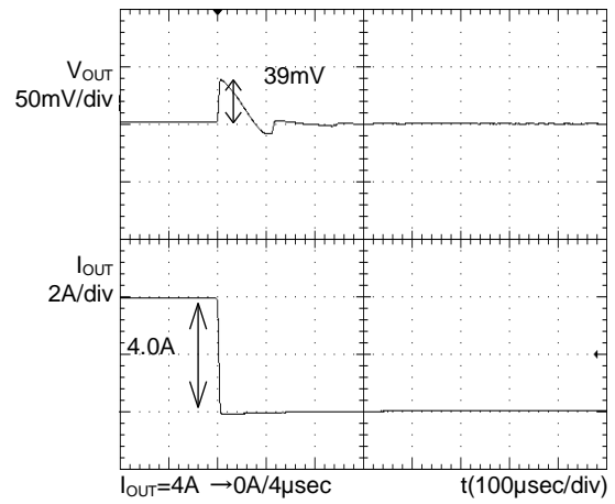
Figure 6. Transient Response (4A → 0A) C_{OUT}=47\mu F, C_{FB}=0.01\mu F
