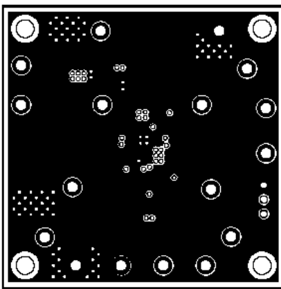
Middle Layer_1
