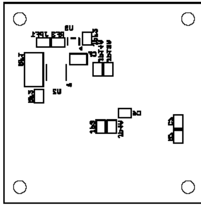
Middle Layer_2
