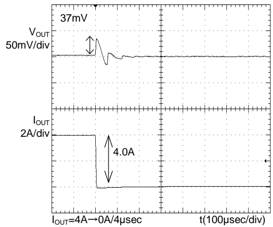
Figure 4. Transient Response (4A → 0A) C_{OUT}=22\mu F, C_{FB}=0.01\mu F
