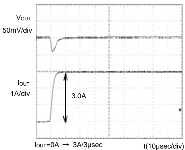
Figure 1. Transient Response (0A → 3A) C_{OUT}=22\mu F , C_{FB}=1000pF
