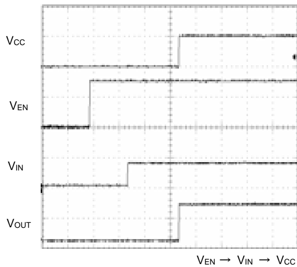
Figure 14. Input Sequence
