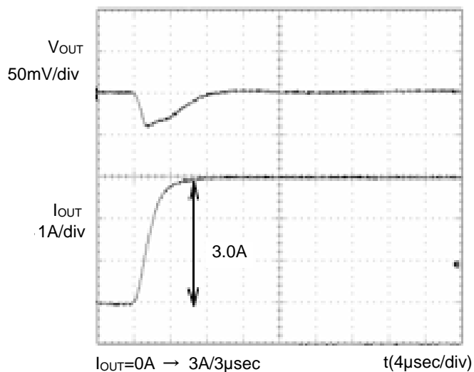
Figure 2. Transient Response (0A → 3A) C_{OUT}=100\mu F
