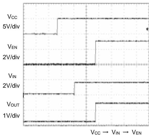
Figure 9. Input Sequence
