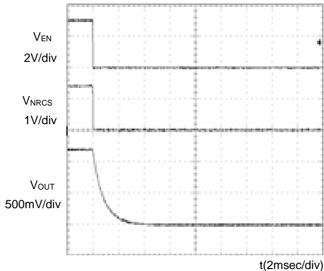
Figure 8. Waveform at Output OFF
