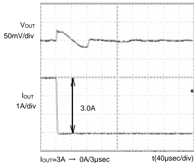
Figure 4. Transient Response (3A → 0A) C_{OUT}=22\mu F , C_{FB}=1000pF
