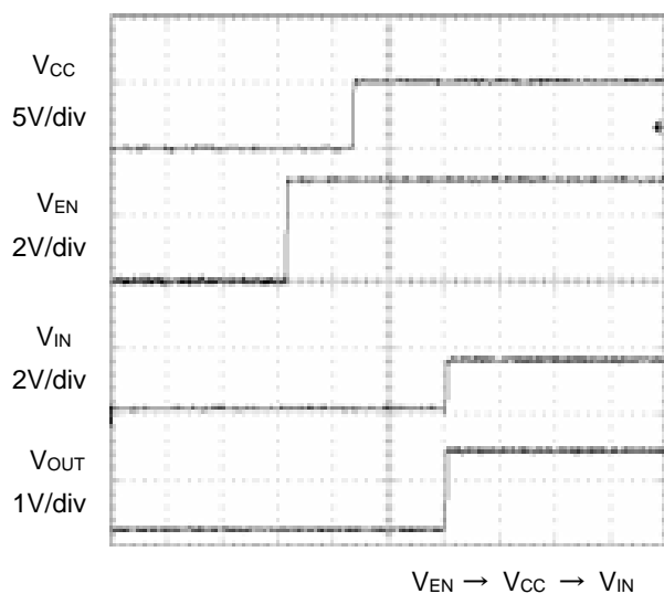
Figure 11. Input Sequence
