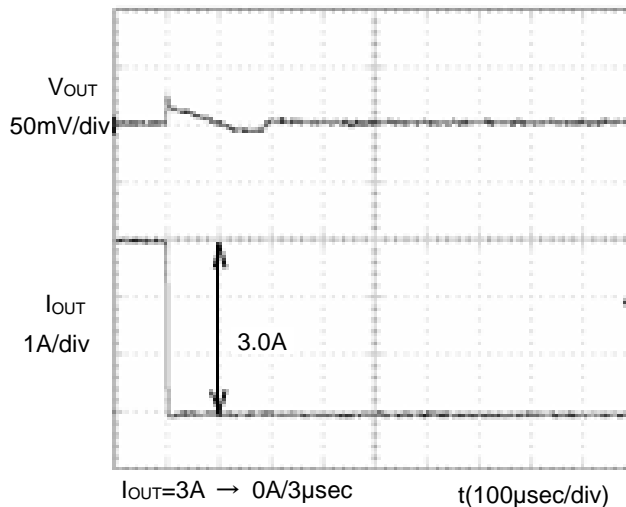
Figure 6. Transient Response (3A → 0A) C_{OUT}=100\mu F, C_{FB}=1000pF
