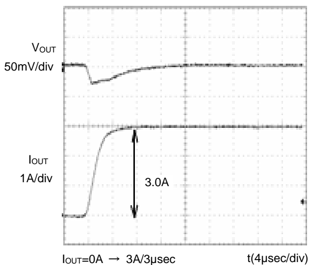
Figure 3. Transient Response (0A → 3A) C_{OUT}=100\mu F , C_{FB}=1000pF
