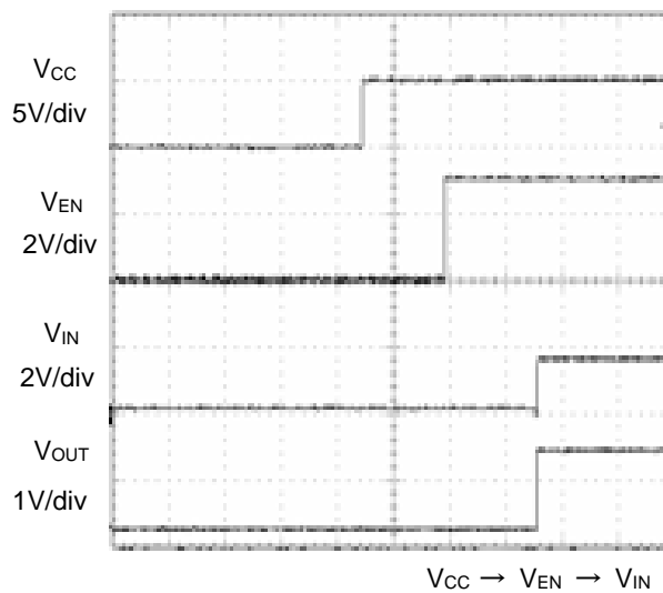
Figure 12. Input Sequence
