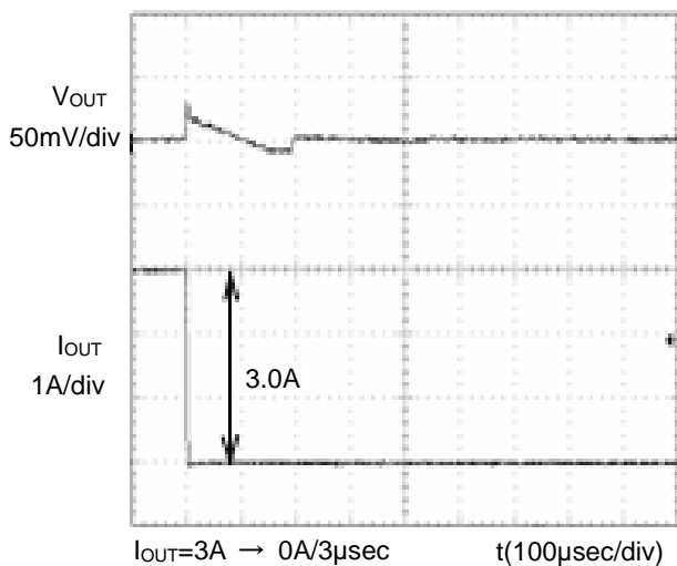
Figure 5. Transient Response (3A → 0A) C_{OUT}=100\mu F
