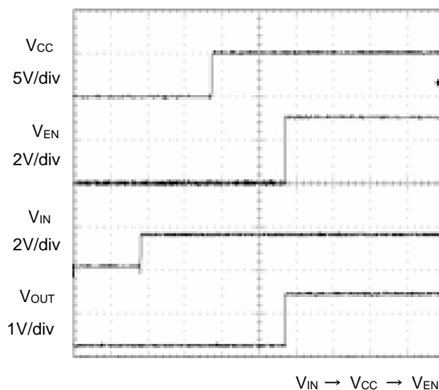
Figure 10. Input Sequence
