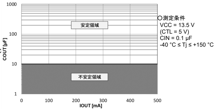
Figure 41. COUT vs 出力電流 (IOUT)
