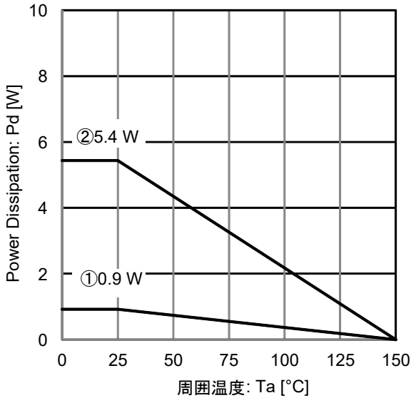
Figure 53. 熱低減曲線グラフ (TO252-3 / TO252-5)
