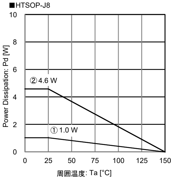
Figure 55. 熱低減曲線グラフ (HTSOP-J8)
