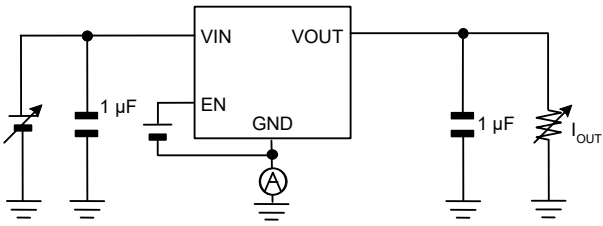
Measurement Setup for Figure 1 to 5, 16, 40 to 44
