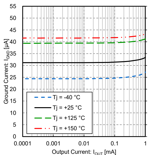
Figure 43. Ground Current vs Output Current; Enlarged view of Figure 42 at low Output Current (3.3 V Output)
