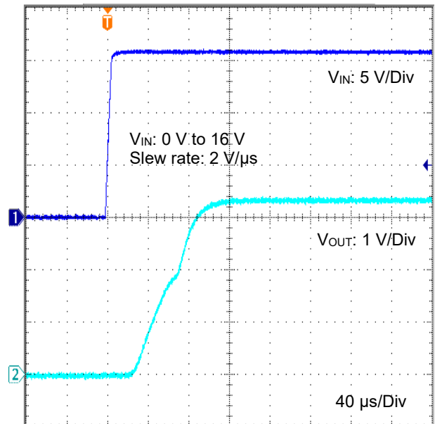
Figure 69. VIN Startup Waveform V_{IN}: 0\text{ V to }16\text{ V} (3.3 V Output, Slew rate = 2\text{ V}/\mu\text{s} , I_{OUT} = 500\text{ mA} )
