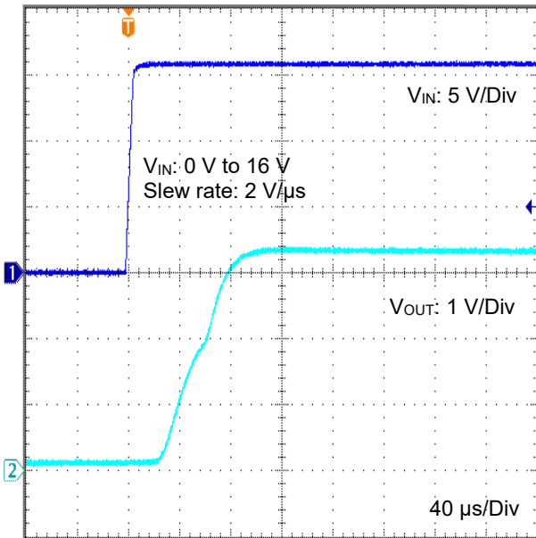
Figure 68. VIN Startup Waveform V_{IN}: 0\text{ V to }16\text{ V} (3.3 V Output, Slew rate = 2\text{ V}/\mu\text{s} , I_{OUT} = 0\text{ mA} )
