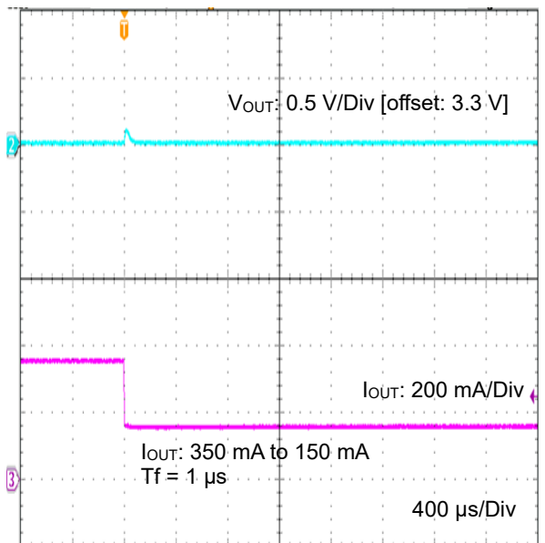
Figure 63. Load Transient 350 mA to 150 mA (3.3 V Output, T_r = 1\text{ }\mu\text{s} , C_{OUT} = 4.7\text{ }\mu\text{F} )
