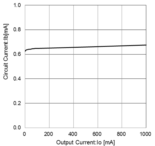
Figure 11. 負荷別回路電流 ( I_o=0mA \rightarrow 1000 mA )
