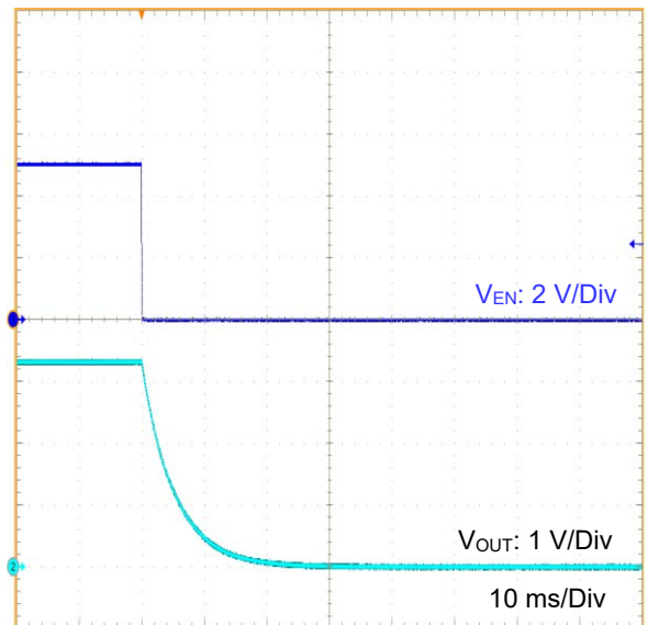
Figure 54. V_{EN} Shutdown Waveform (3.3 V Output, I_{OUT} = 1\text{ mA} )
