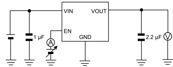
Measurement Setup for Figure 17, 18
