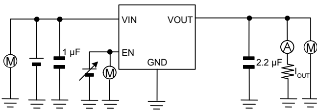
Measurement Setup for Figure 29, 30, 53, 54
