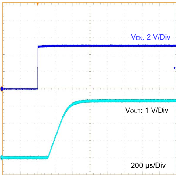
Figure 53. V_{EN} Startup Waveform (3.3 V Output, I_{OUT} = 1\text{ mA} )
