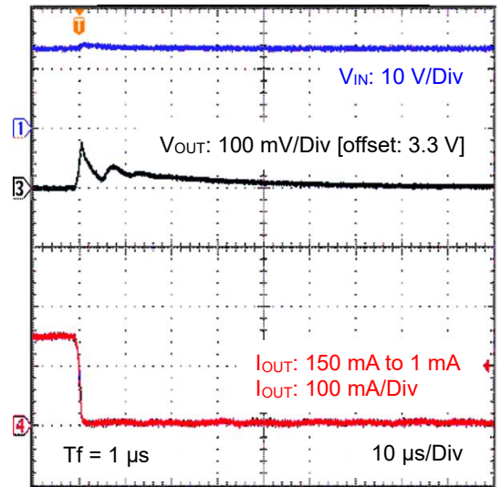
Figure 42. Load Transient 150 mA to 1 mA (3.3 V output, T_f = 1\text{ }\mu\text{s} )
