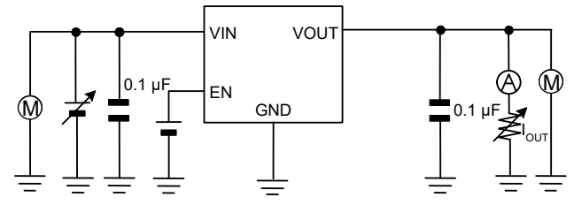
Measurement Setup for Figure 19 to 26, 41 to 48
