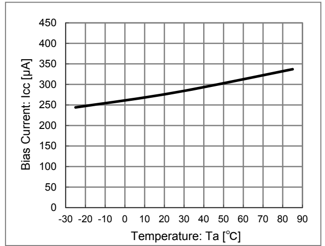
Figure 7. Ta - Icc
