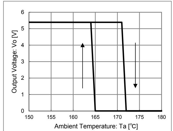
Figure ure 11. TSD ( I_o = 0\text{mA} )
