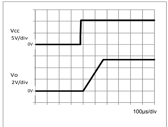
Figure 3. Input sequence (C OUT = 1μF)
