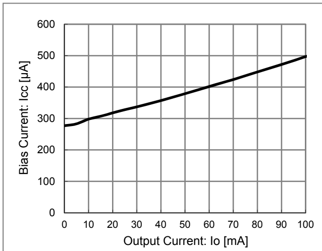
Figure 8. I o - Icc
