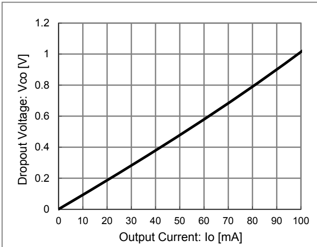
Figure 10. Minimum dropout Voltage
