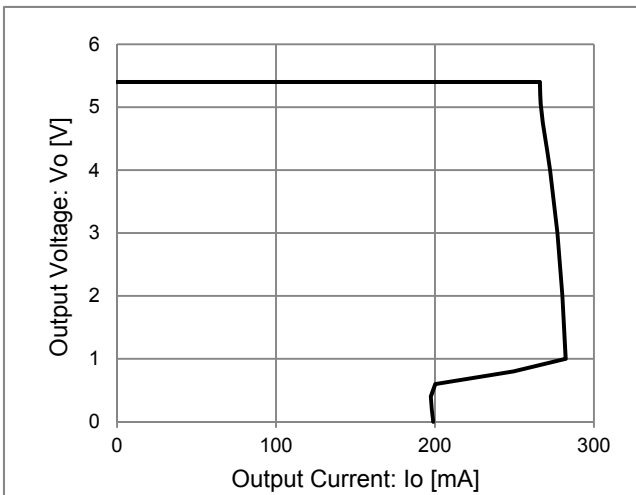
Figure 12. OCP
